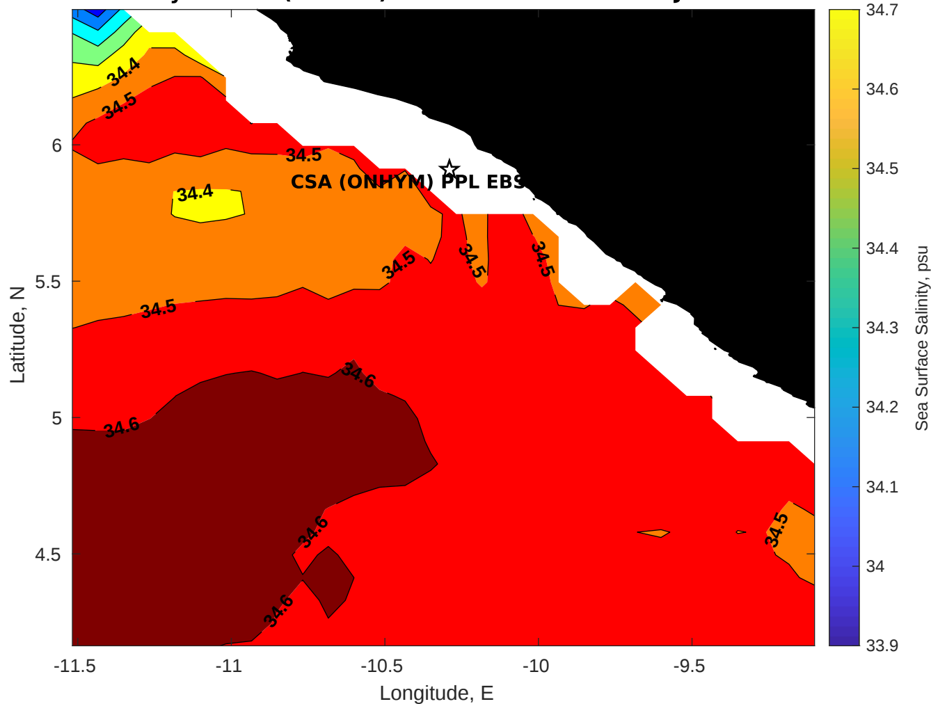
Surface Salinity for CSA (ONHYM) PPL EBS - Liberia at 13-Jan-2026 00:00:00
