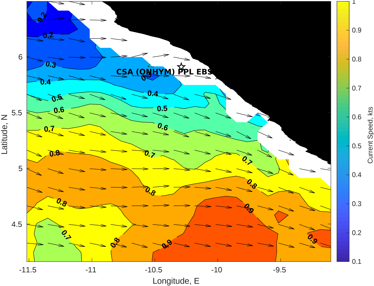
Surface Currents for CSA (ONHYM) PPL EBS - Liberia at 13-Jan-2026 00:00:00
