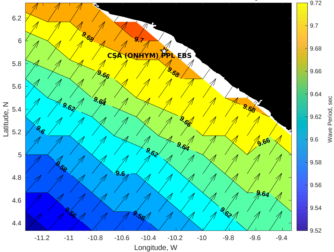
GFS Wave Period (sec) for CSA (ONHYM) PPL EBS - Liberia at 14-Jan-2026 09:00:00
