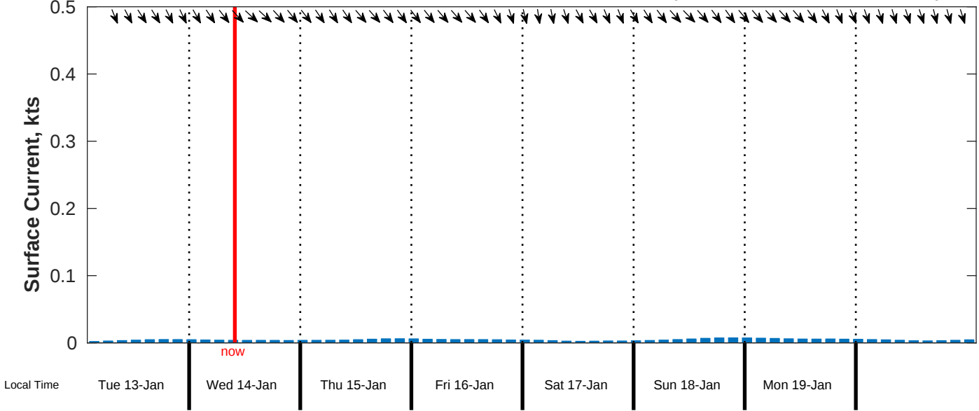
Surface Current Forecast for CSA (ONHYM) PPL EBS - Liberia from 13-Jan-2026 00:00:00 to 21-Jan-2026 00:00:00
