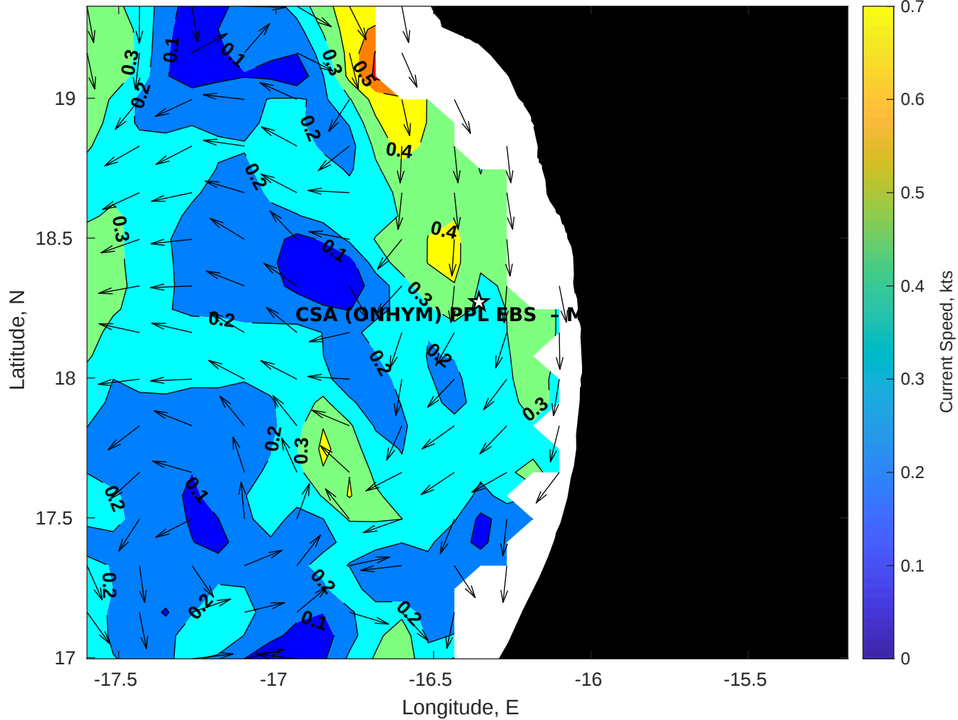
Surface Currents for CSA (ONHYM) PPL EBS - Mauritania at 13-Jan-2026 00:00:00
