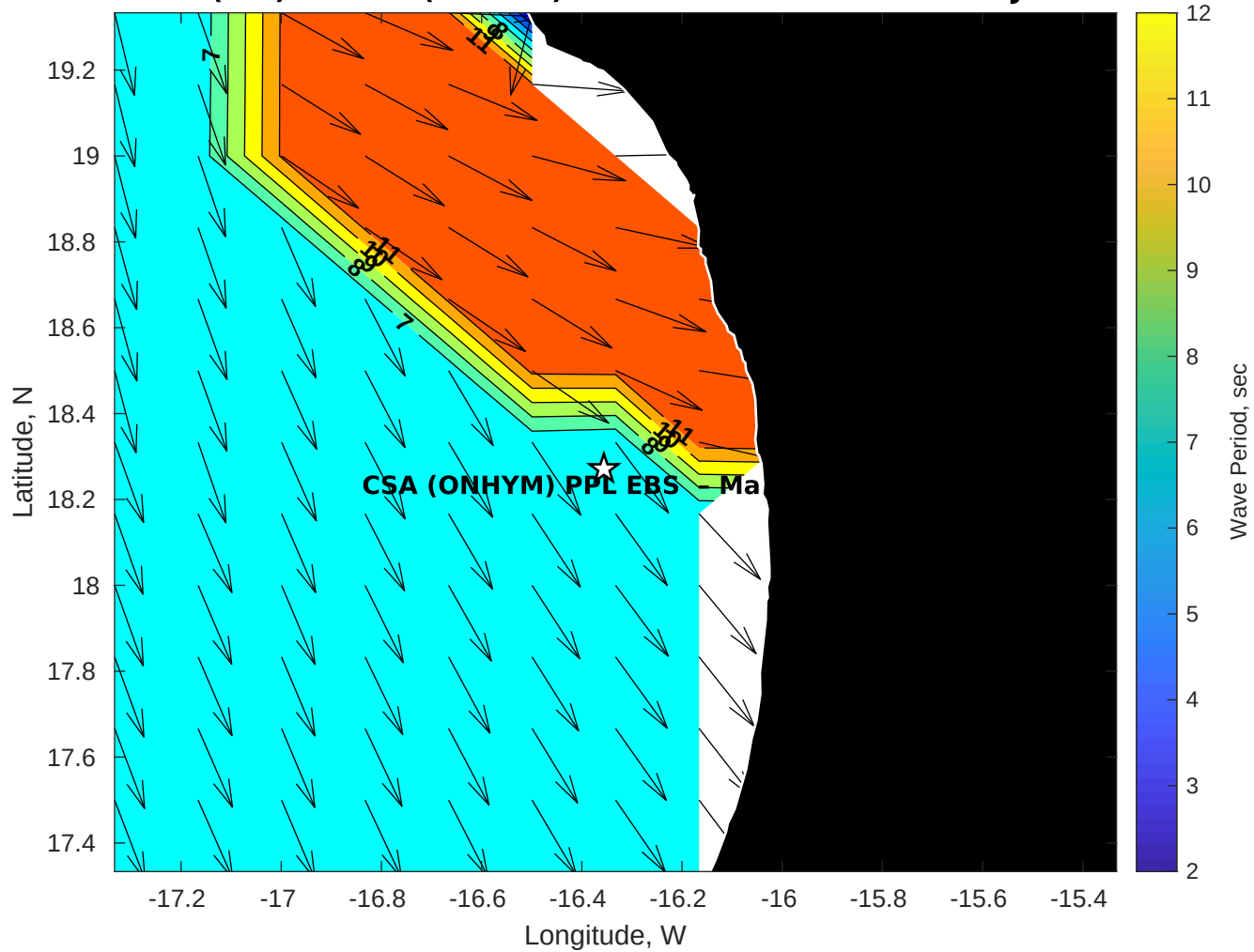
GFS Wave Period (sec) for CSA (ONHYM) PPL EBS - Mauritania at 14-Jan-2026 09:00:00
