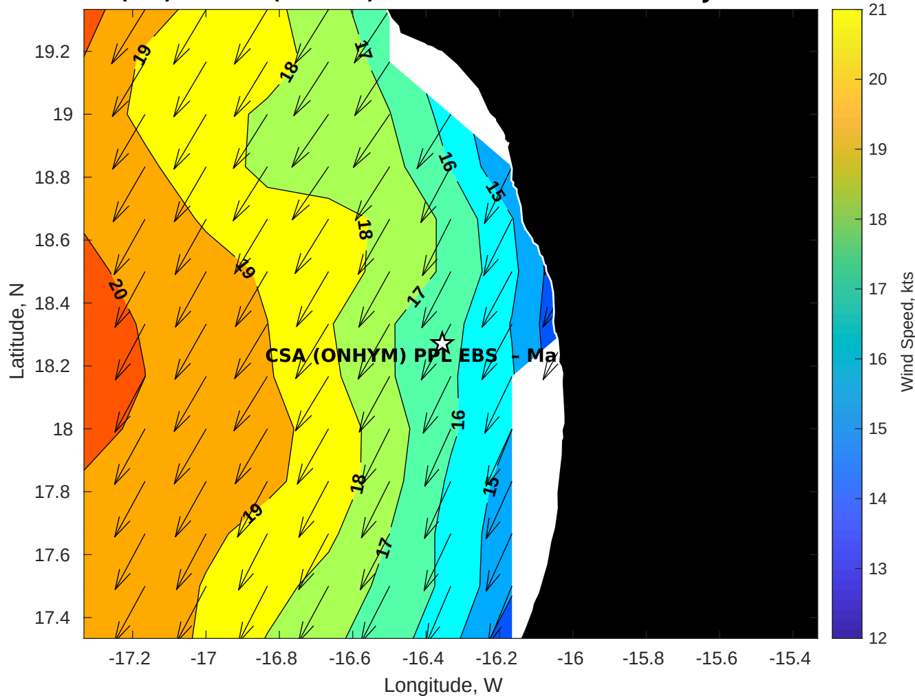
GFS Winds (kts) for CSA (ONHYM) PPL EBS - Mauritania at 14-Jan-2026 09:00:00
