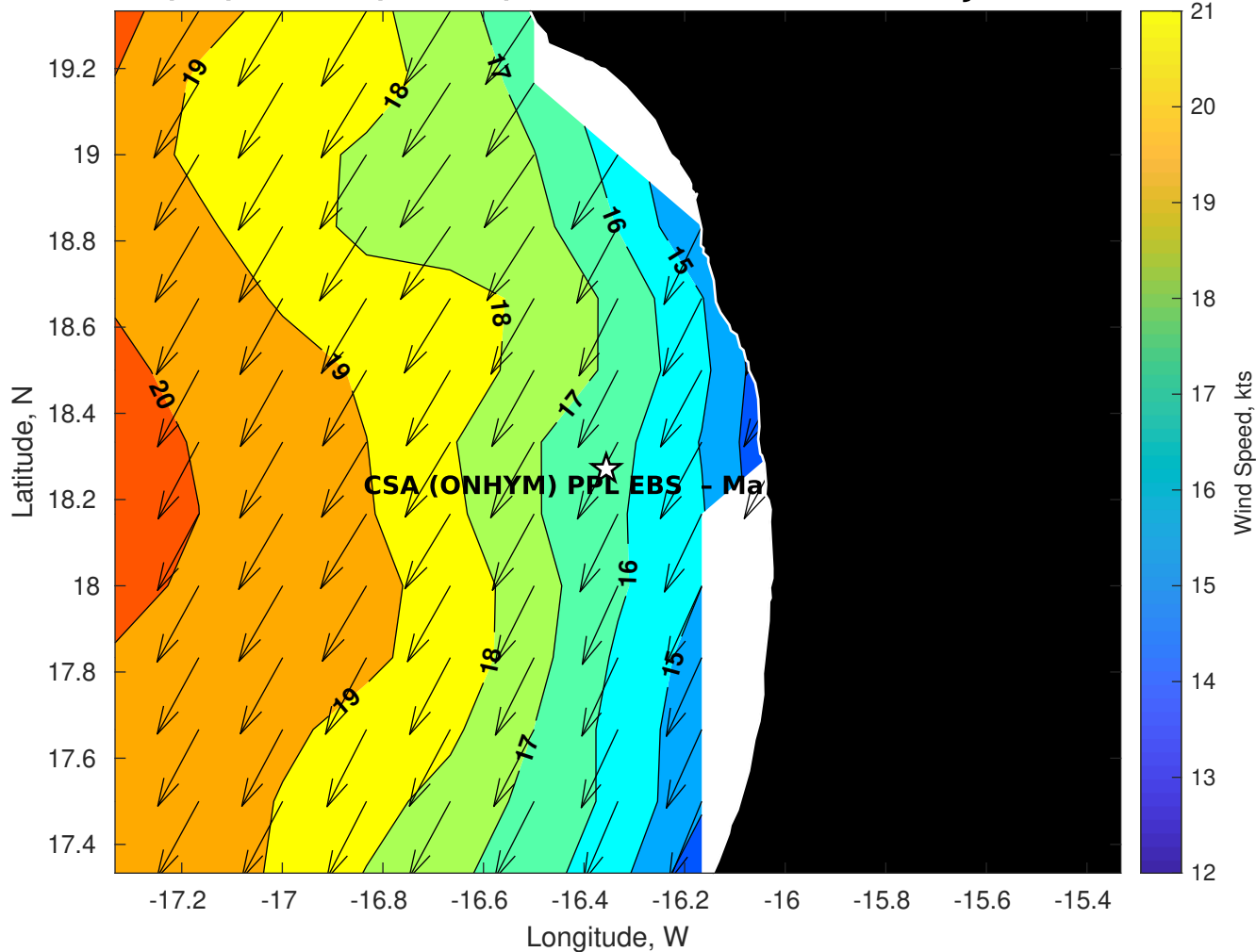
GFS Winds (kts) for CSA (ONHYM) PPL EBS - Mauritania at 14-Jan-2026 09:00:00
