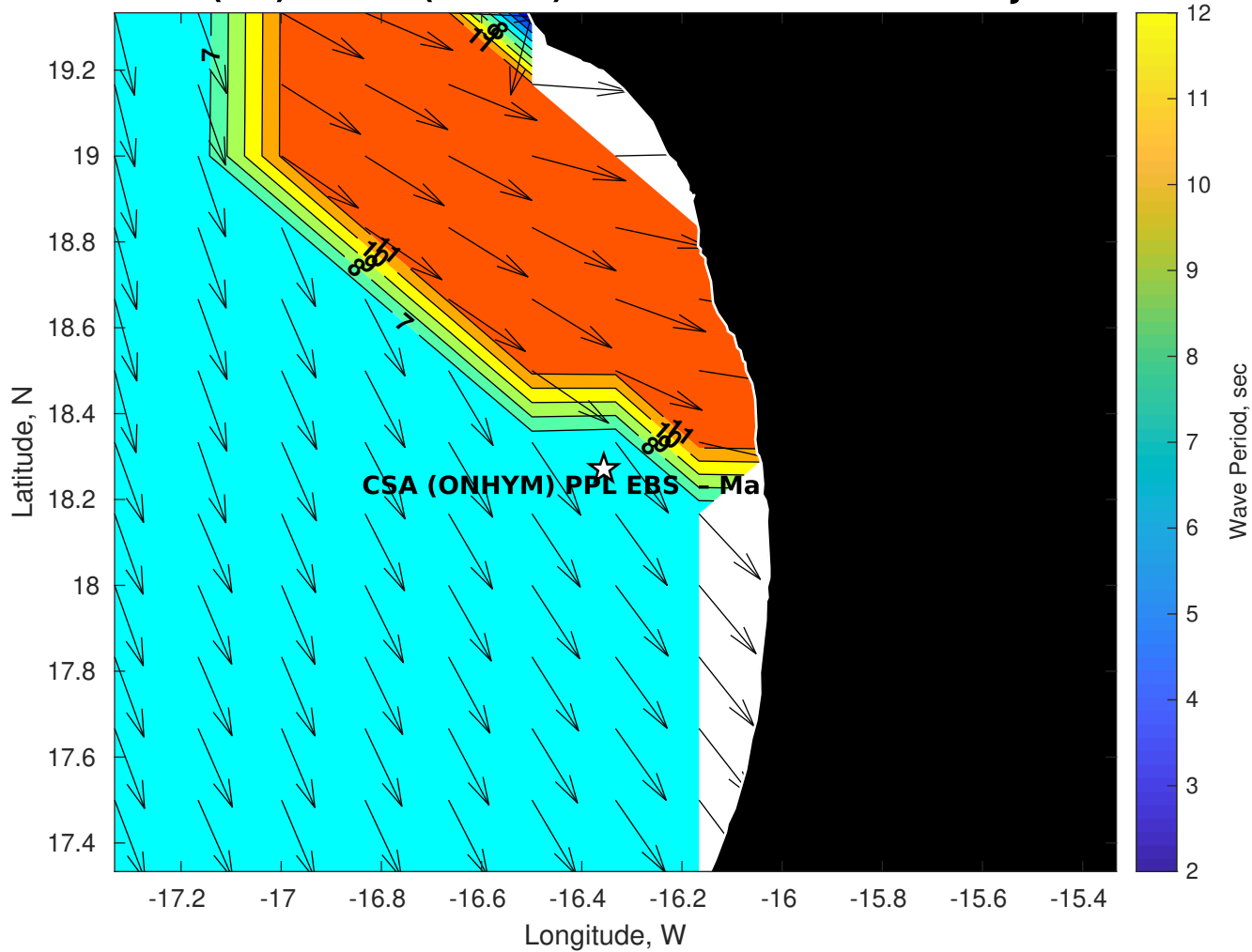
GFS Wave Period (sec) for CSA (ONHYM) PPL EBS - Mauritania at 14-Jan-2026 09:00:00
