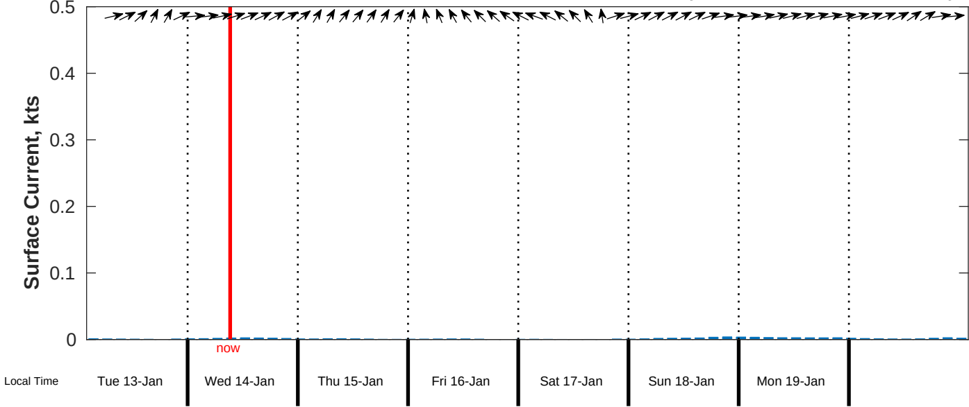
Surface Current Forecast for CSA (ONHYM) PPL EBS - Mauritania from 13-Jan-2026 00:00:00 to 21-Jan-2026 00:00:00
