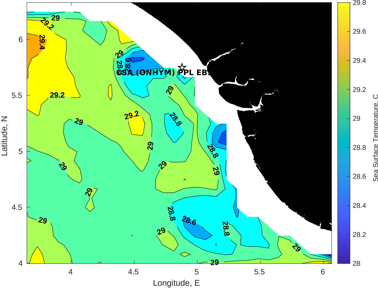
SST for CSA (ONHYM) PPL EBS - Nigeria at 13-Jan-2026 00:00:00
