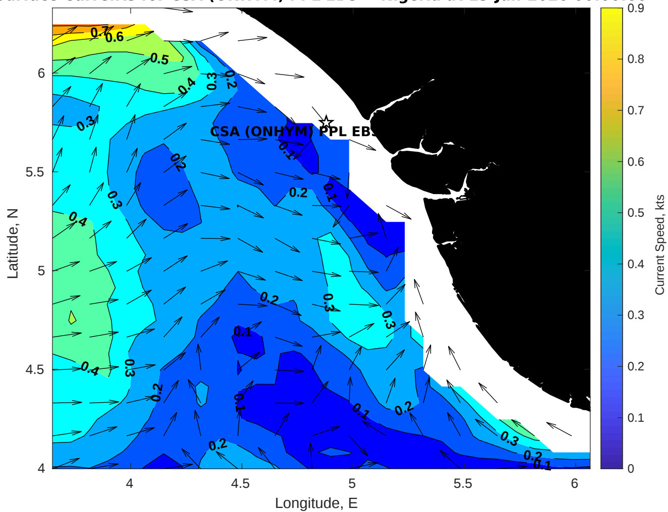
Surface Currents for CSA (ONHYM) PPL EBS - Nigeria at 13-Jan-2026 00:00:00
