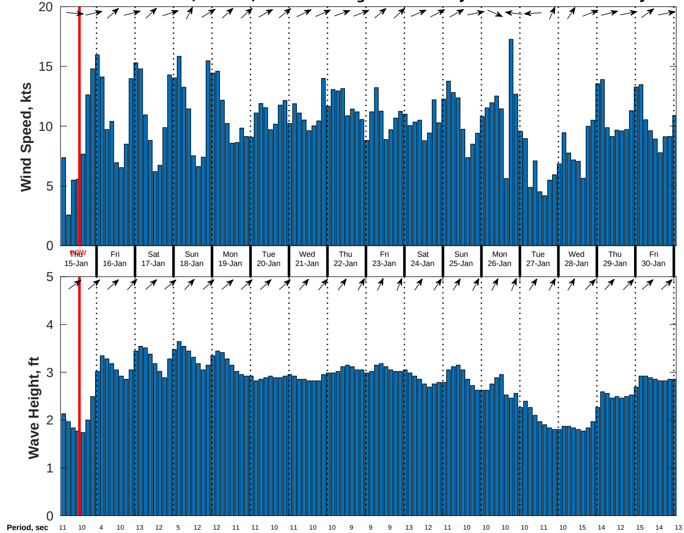
Wind & Wave Forecast for CSA (ONHYM) PPL EBS - Nigeria from 14-Jan-2026 02:00:00 to 30-Jan-2026 02:00:00
