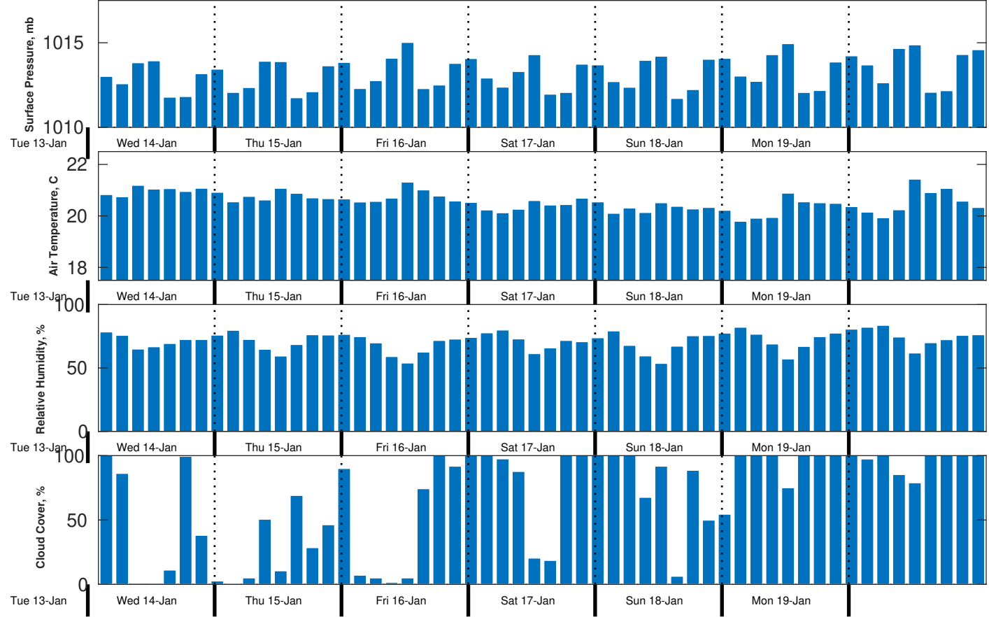
Met Forecast for CSA (ONHYM) PPL EBS - Senegal from 14-Jan-2026 00:00:00 to 21-Jan-2026 00:00:00
