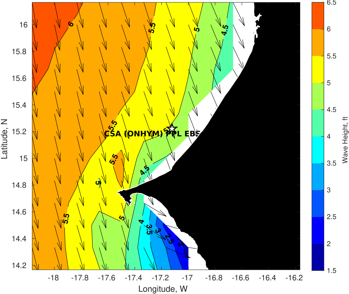
GFS Wave Height (ft) for CSA (ONHYM) PPL EBS - Senegal at 14-Jan-2026 09:00:00
