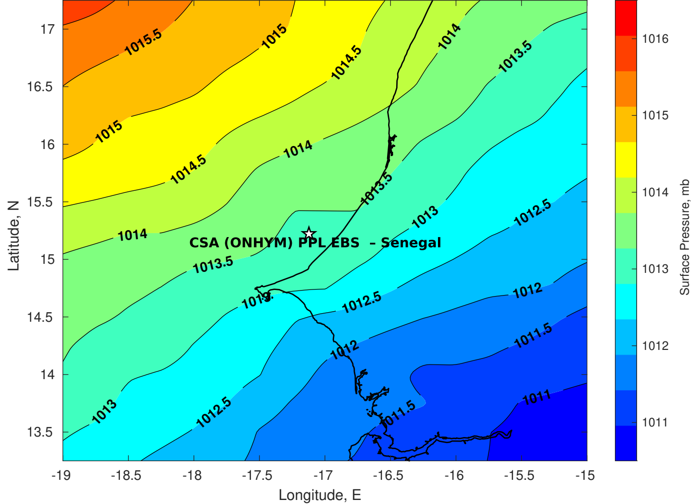
Surface Pressure (mb) for CSA (ONHYM) PPL EBS - Senegal at 15-Jan-2026 00:00:00
