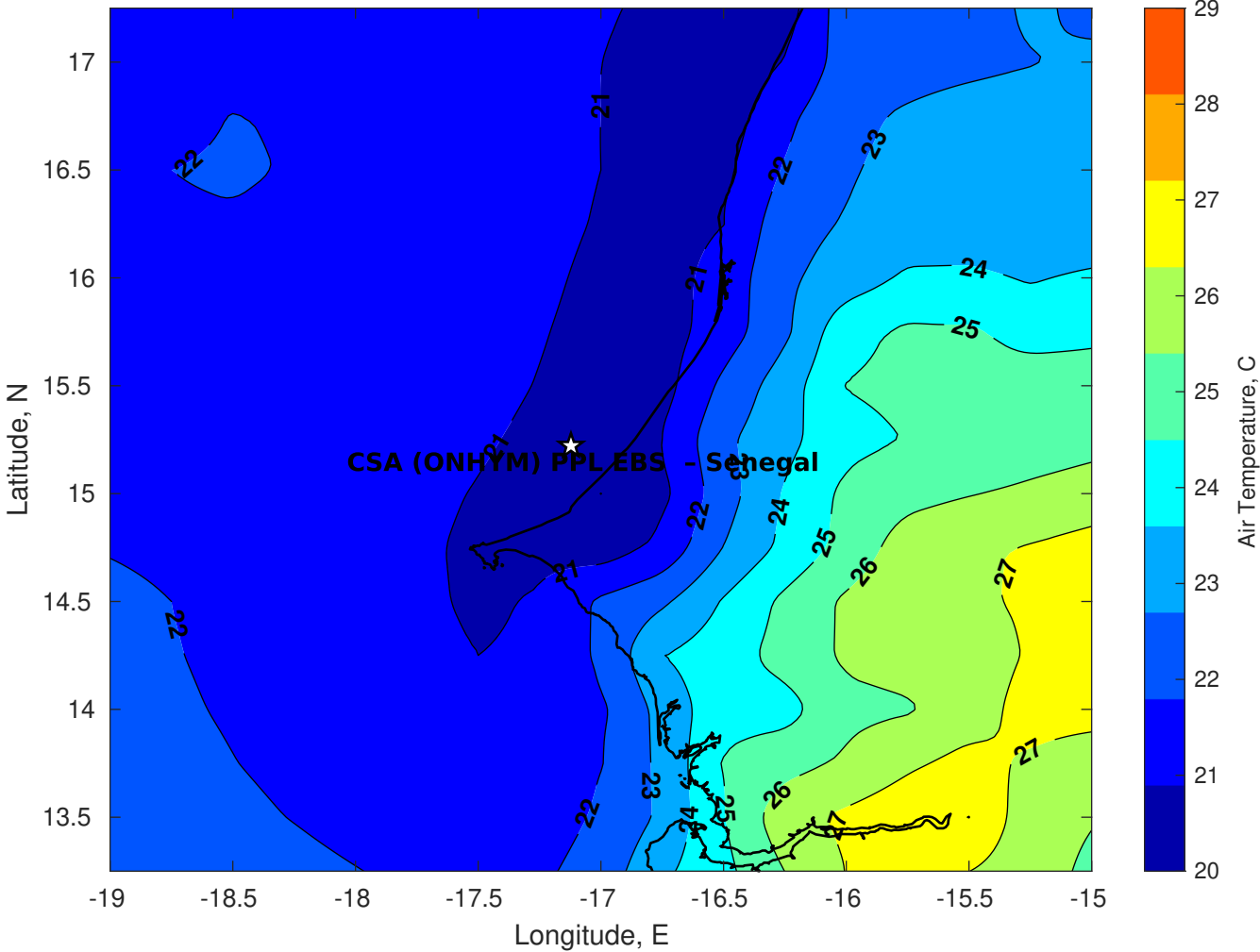
Air Temperature (C) for CSA (ONHYM) PPL EBS - Senegal at 14-Jan-2026
