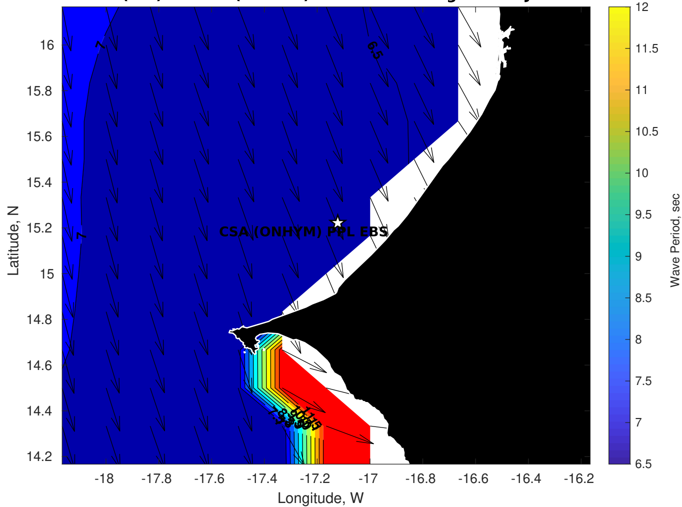
GFS Wave Period (sec) for CSA (ONHYM) PPL EBS - Senegal at 14-Jan-2026 09:00:00
