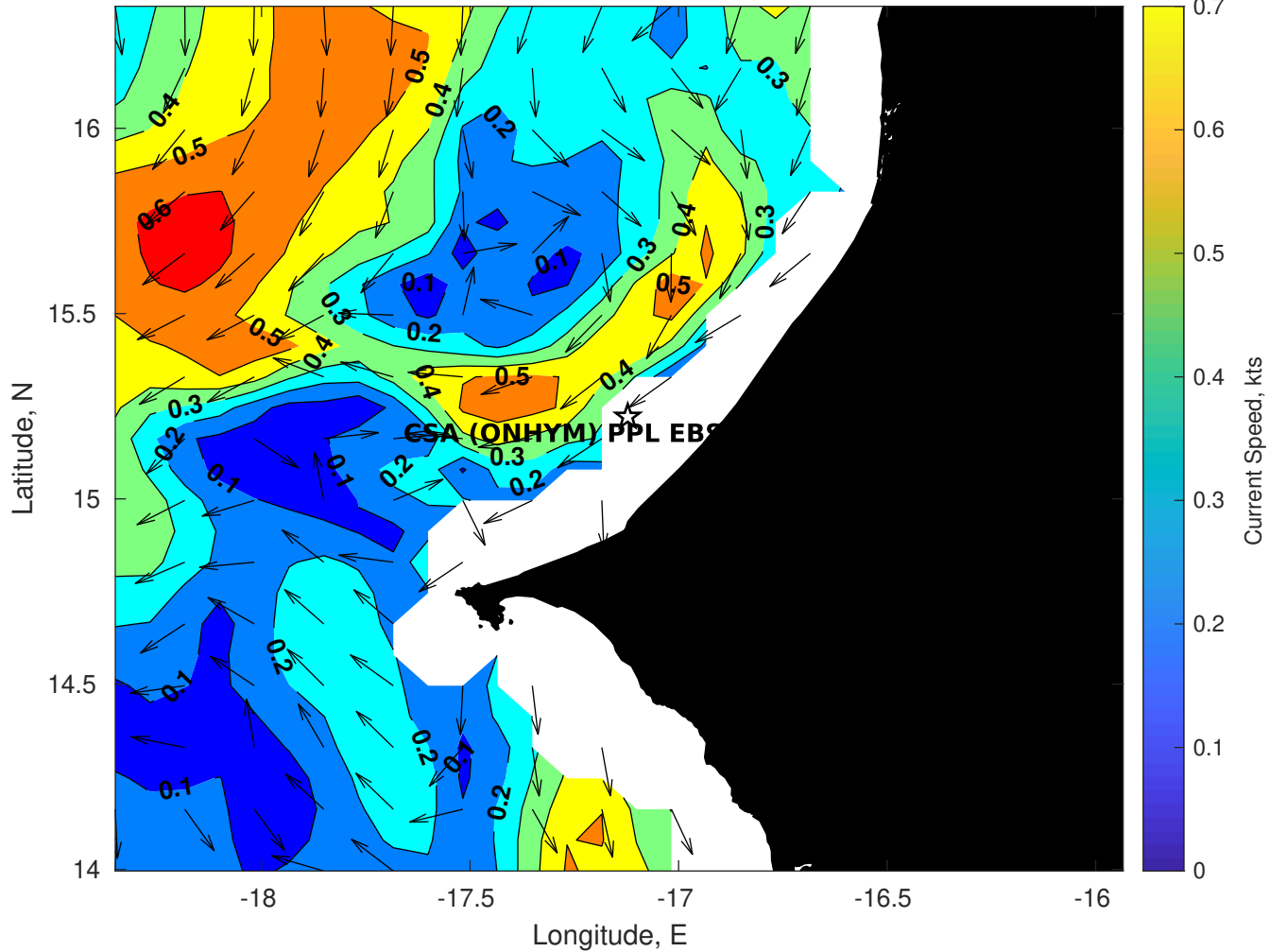
Surface Currents for CSA (ONHYM) PPL EBS - Senegal at 13-Jan-2026 00:00:00
