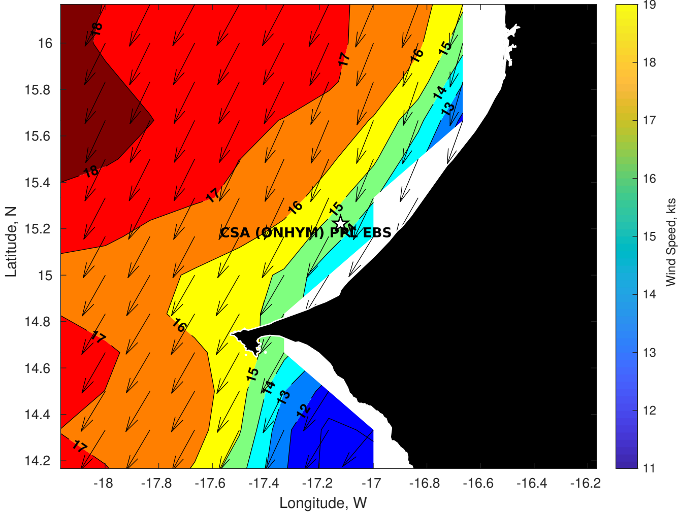
GFS Winds (kts) for CSA (ONHYM) PPL EBS - Senegal at 14-Jan-2026 09:00:00
