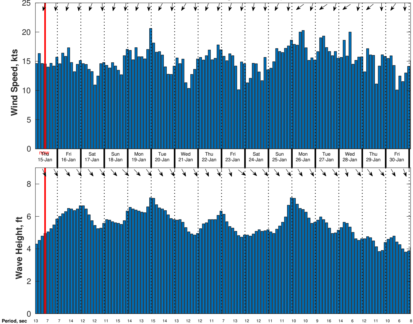
Wind & Wave Forecast for CSA (ONHYM) PPL EBS - Senegal from 14-Jan-2026 01:00:00 to 30-Jan-2026 01:00:00
