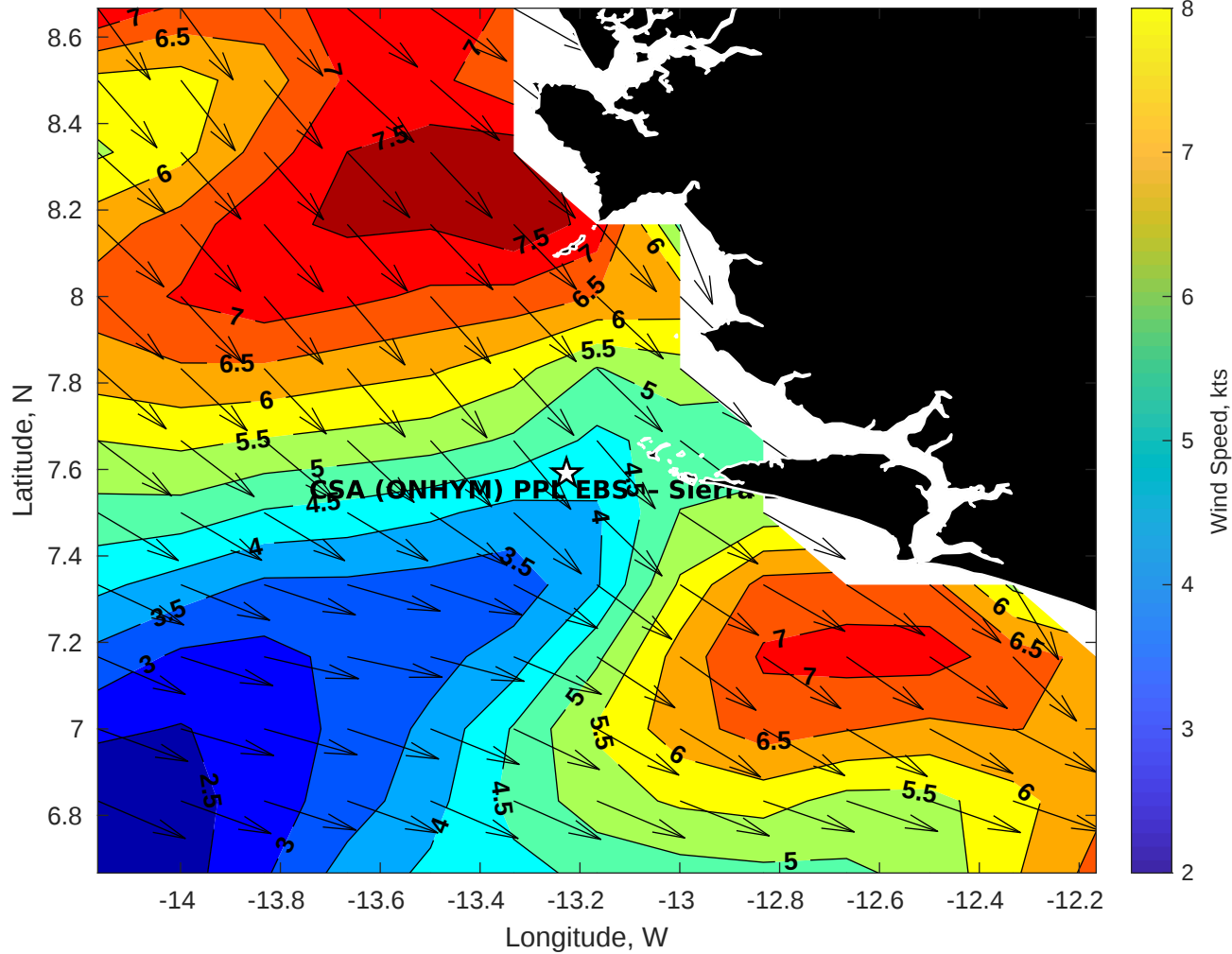
GFS Winds (kts) for CSA (ONHYM) PPL EBS - Sierra Leone at 14-Jan-2026 09:00:00
