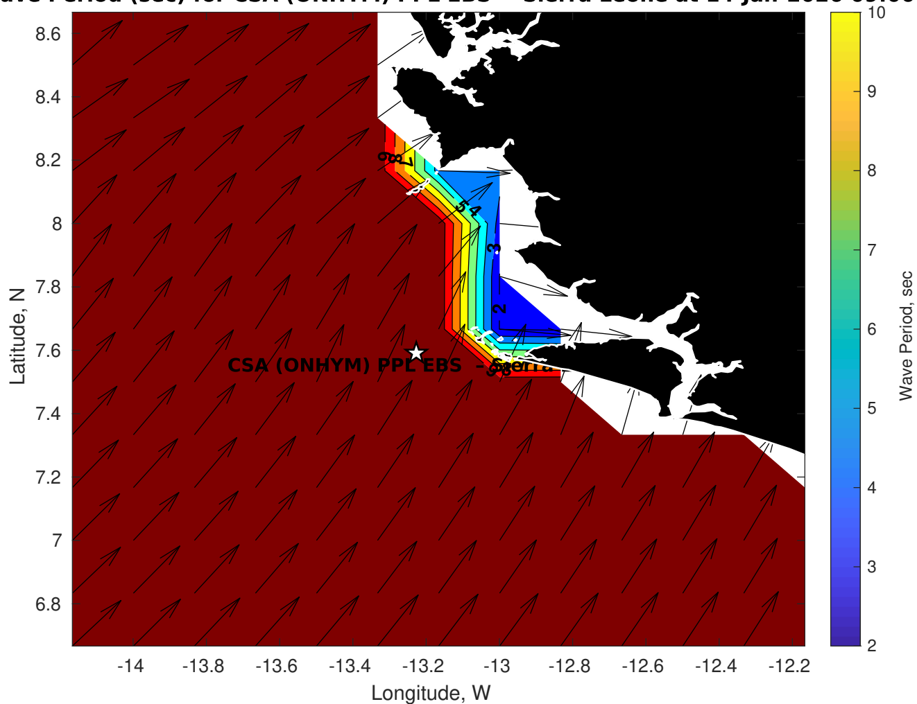
GFS Wave Period (sec) for CSA (ONHYM) PPL EBS - Sierra Leone at 14-Jan-2026 09:00:00
