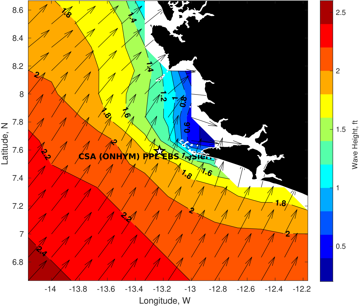
GFS Wave Height (ft) for CSA (ONHYM) PPL EBS - Sierra Leone at 14-Jan-2026 09:00:00
