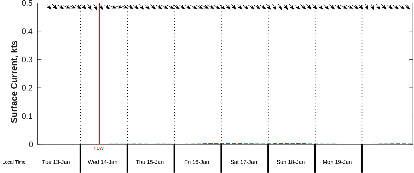
Surface Current Forecast for CSA (ONHYM) PPL EBS - Sierra Leone from 13-Jan-2026 00:00:00 to 21-Jan-2026 00:00:00
