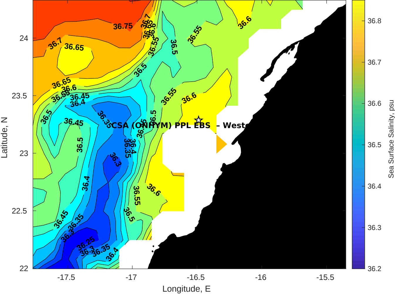
Surface Salinity for CSA (ONHYM) PPL EBS - Western Sahara at 13-Jan-2026 00:00:00
