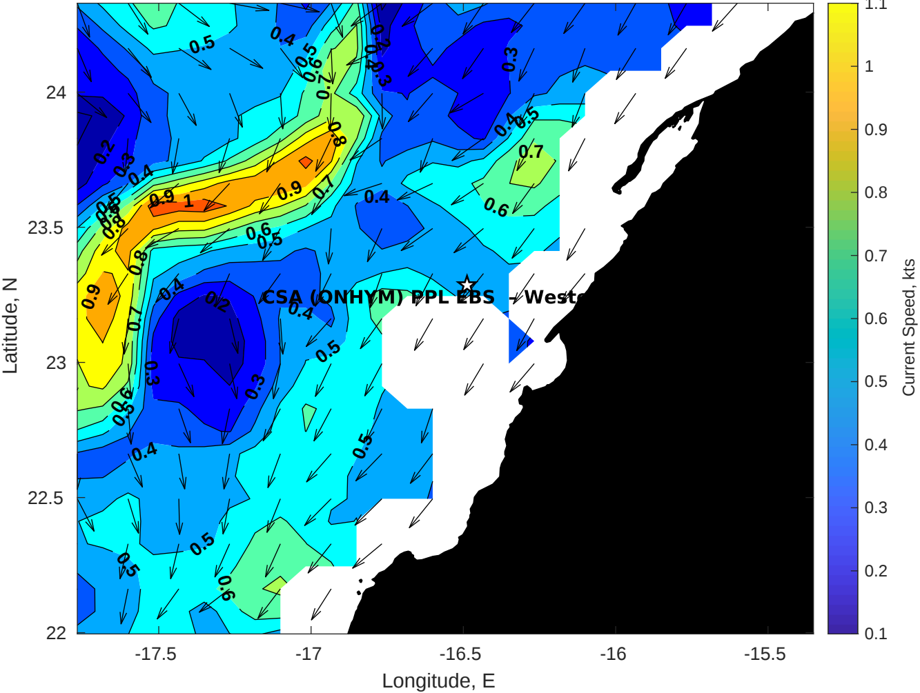
Surface Currents for CSA (ONHYM) PPL EBS - Western Sahara at 13-Jan-2026 00:00:00
