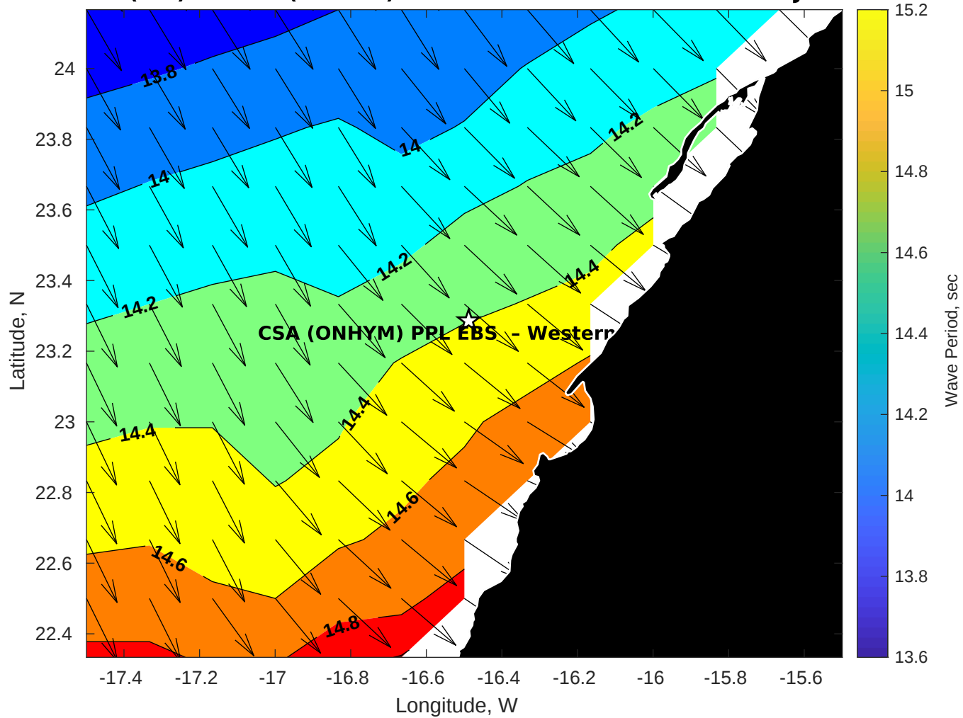
GFS Wave Period (sec) for CSA (ONHYM) PPL EBS - Western Sahara at 14-Jan-2026 09:00:00
