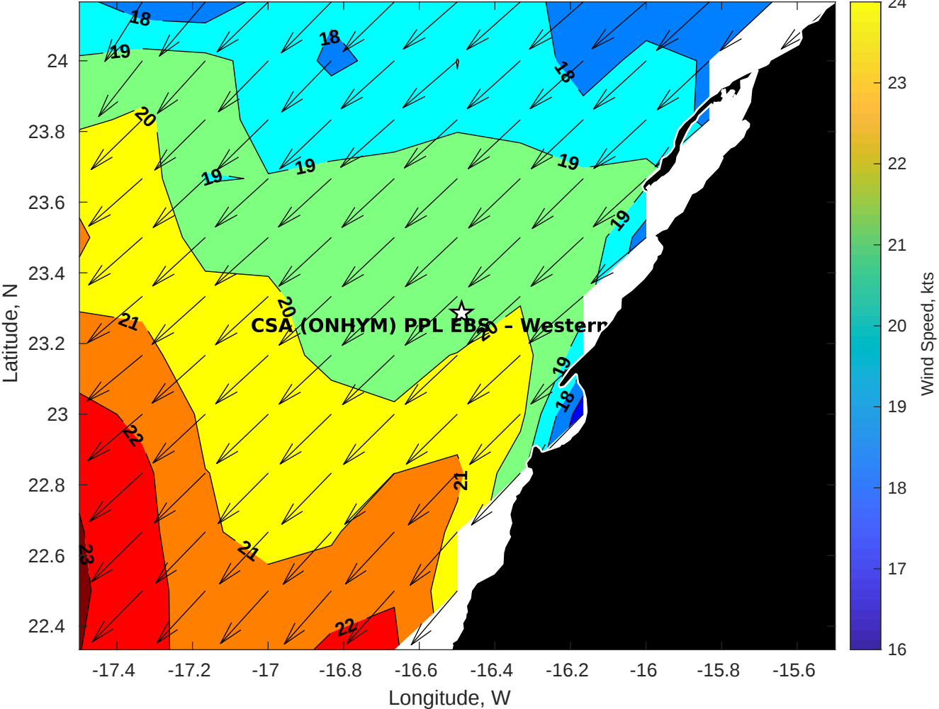
GFS Winds (kts) for CSA (ONHYM) PPL EBS - Western Sahara at 14-Jan-2026 09:00:00
