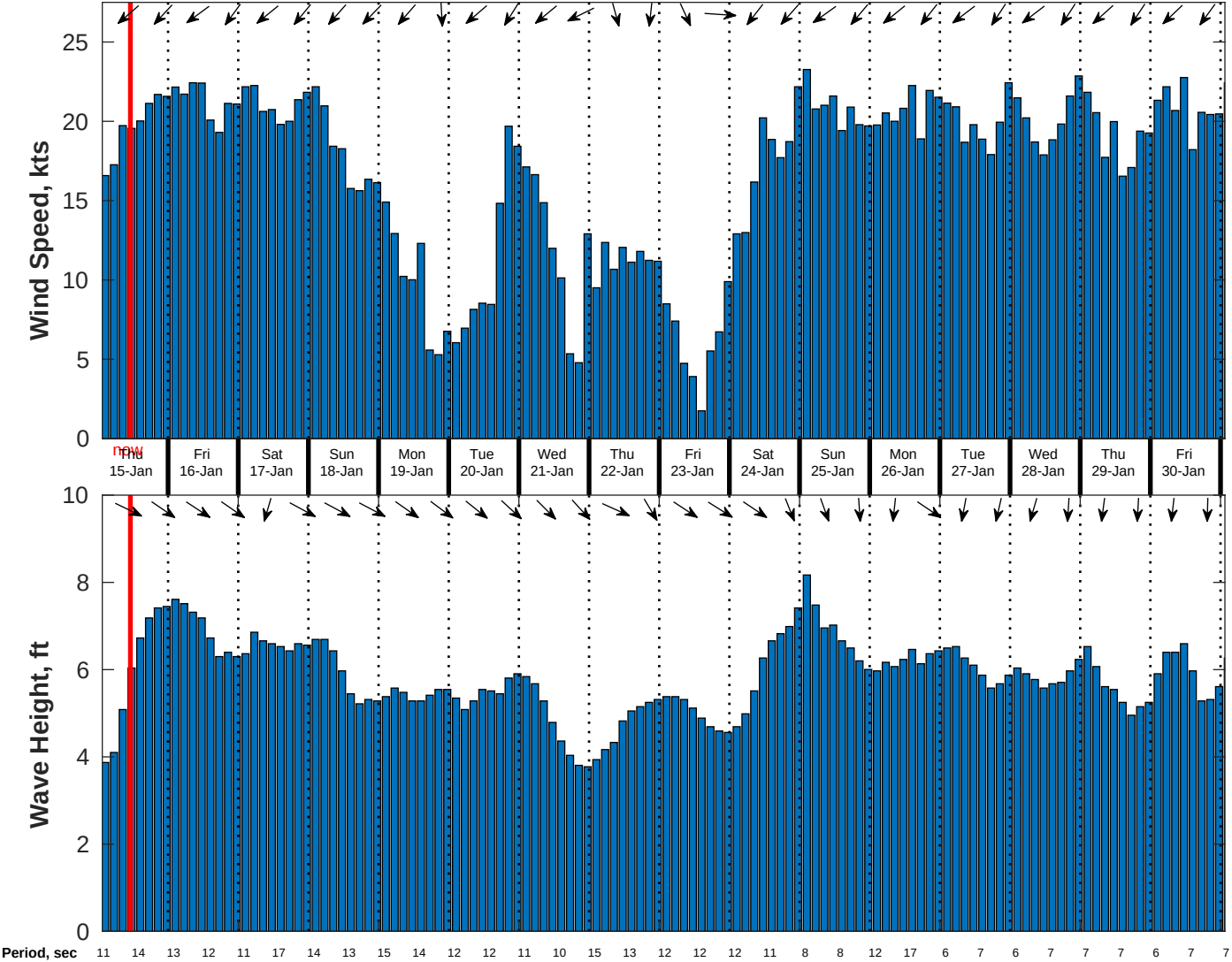
Wind & Wave Forecast for CSA (ONHYM) PPL EBS - Western Sahara from 14-Jan-2026 01:00:00 to 30-Jan-2026 01:00:00
