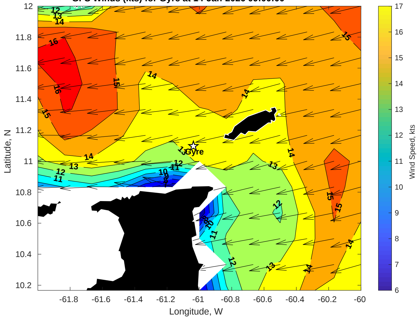
GFS Winds (kts) for Gyre at 14-Jan-2026 09:00:00
