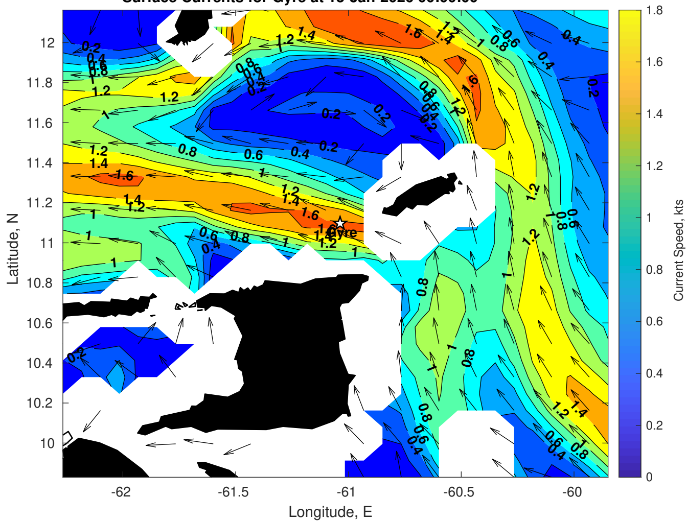
Surface Currents for Gyre at 13-Jan-2026 00:00:00
