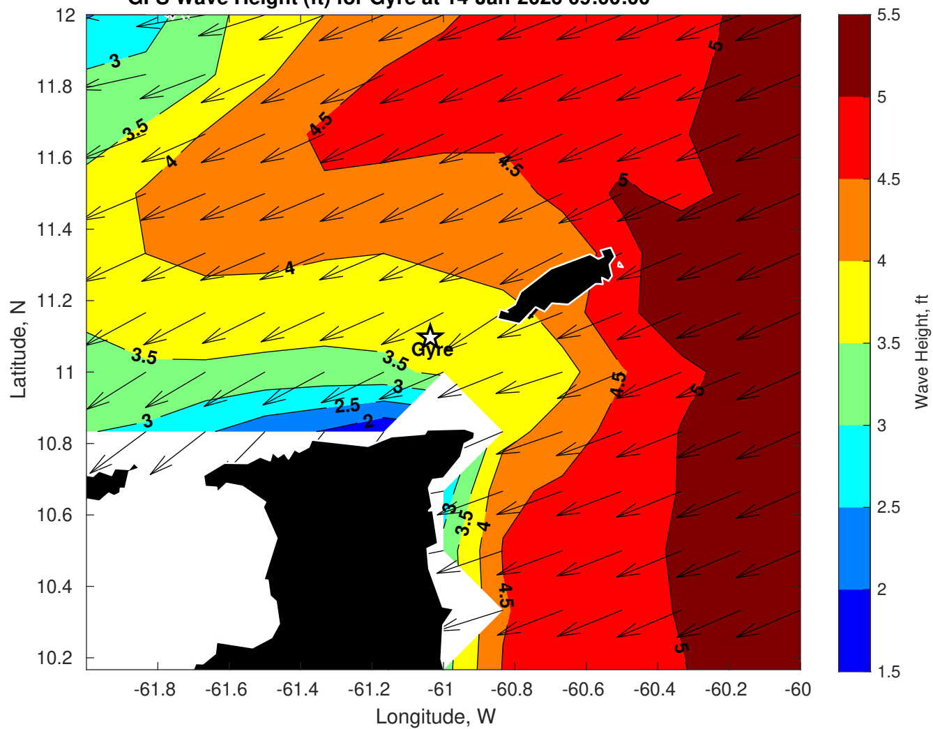
GFS Wave Height (ft) for Gyre at 14-Jan-2026 09:00:00
