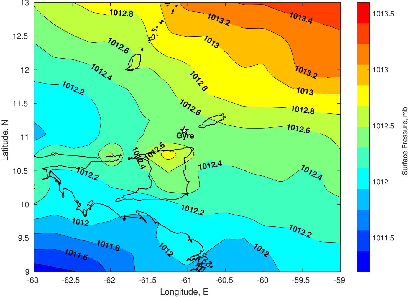
Surface Pressure (mb) for Gyre at 15-Jan-2026 00:00:00
