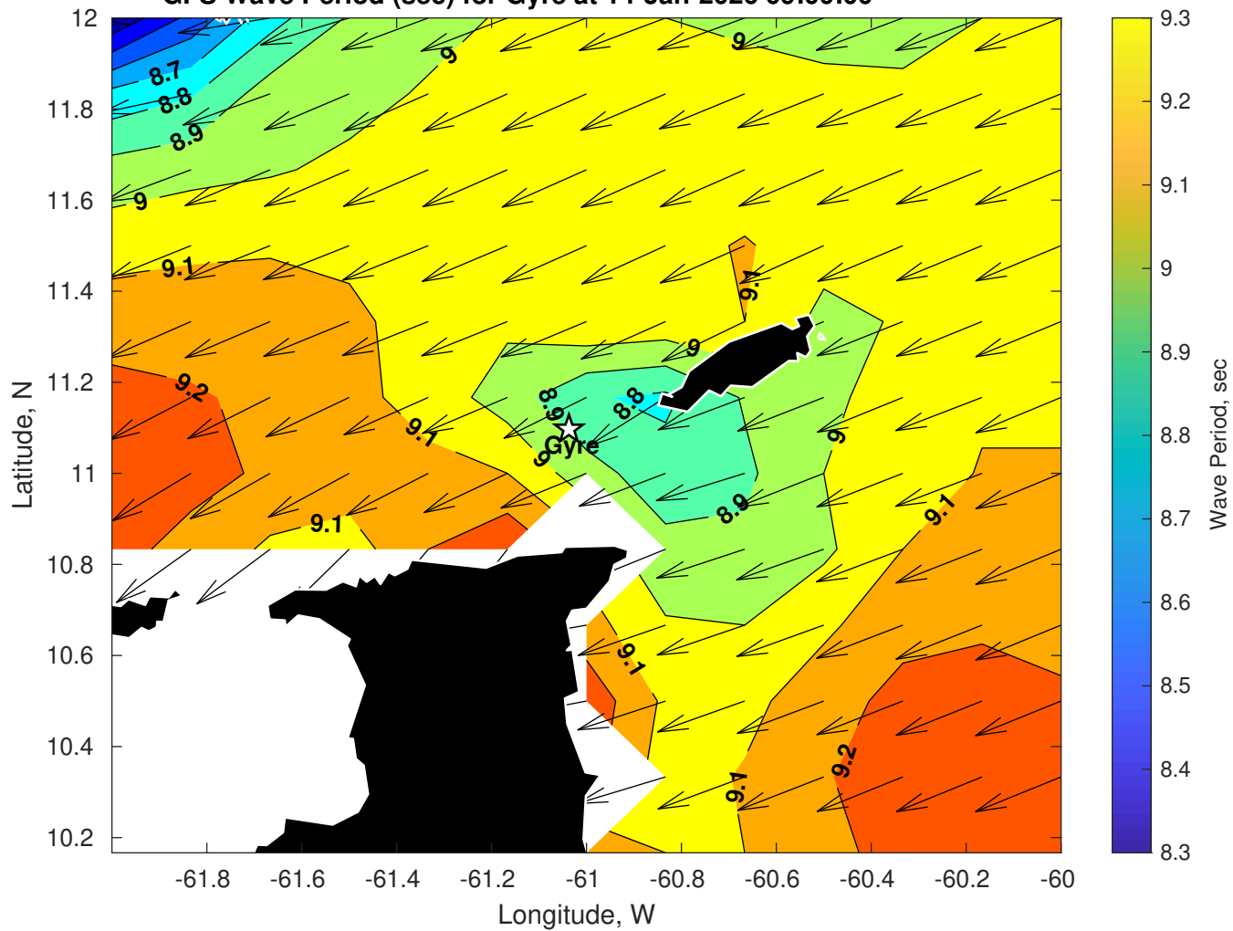
GFS Wave Period (sec) for Gyre at 14-Jan-2026 09:00:00
