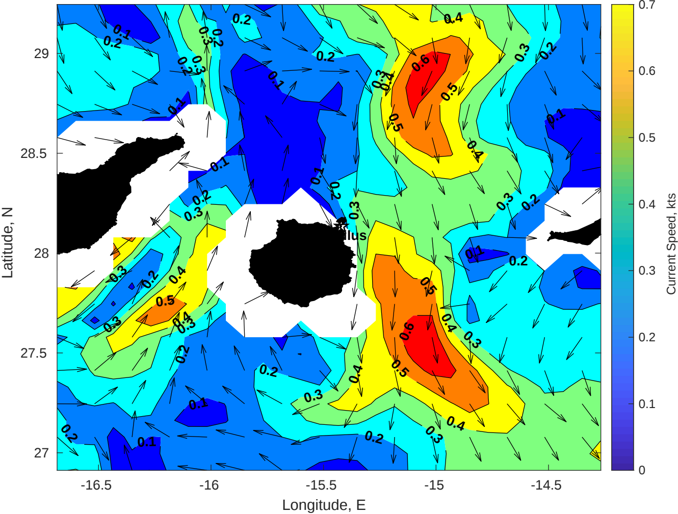
Surface Currents for Nautilus at 13-Jan-2026 00:00:00
