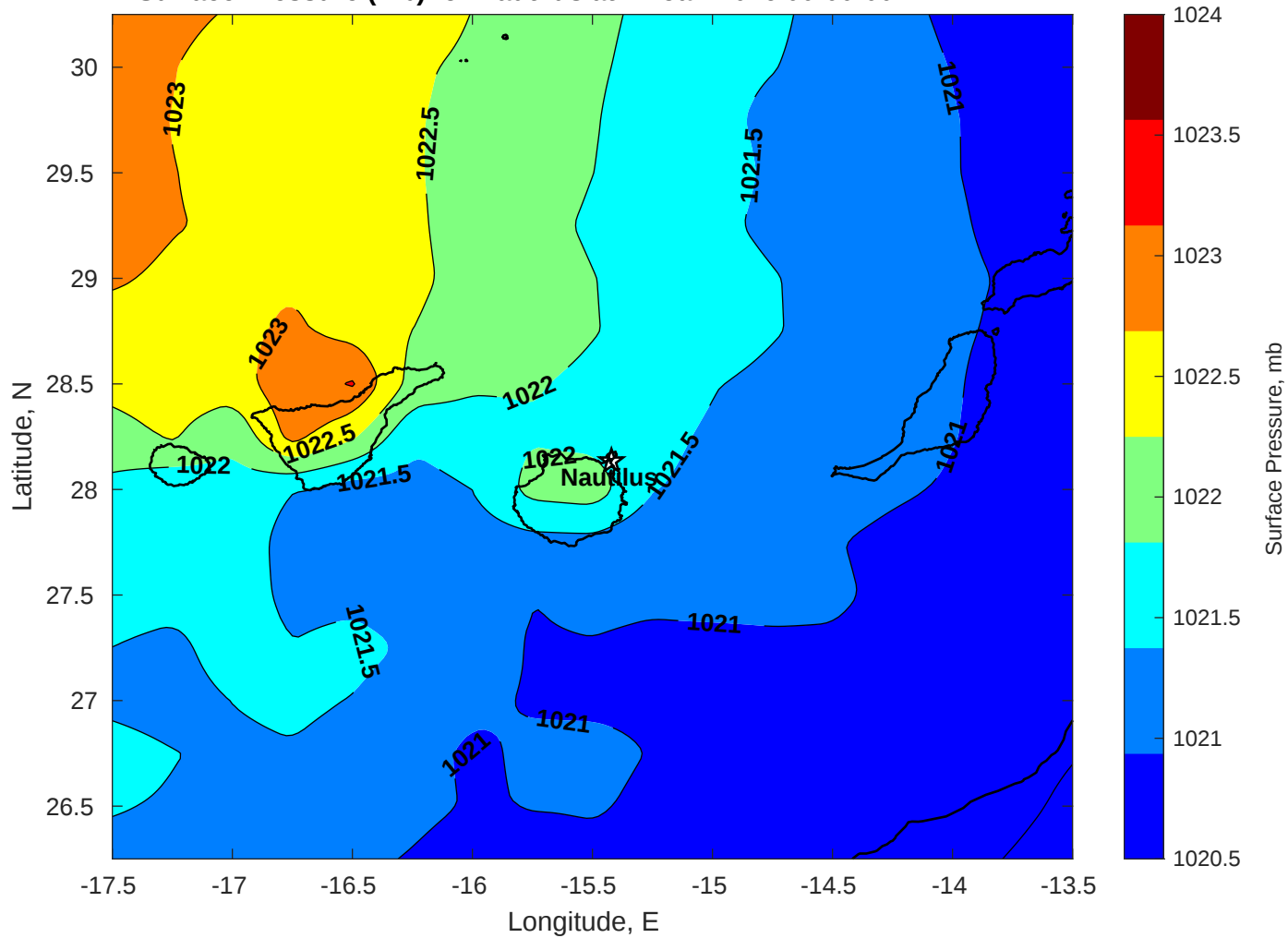
Surface Pressure (mb) for Nautilus at 14-Jan-2026 00:00:00
