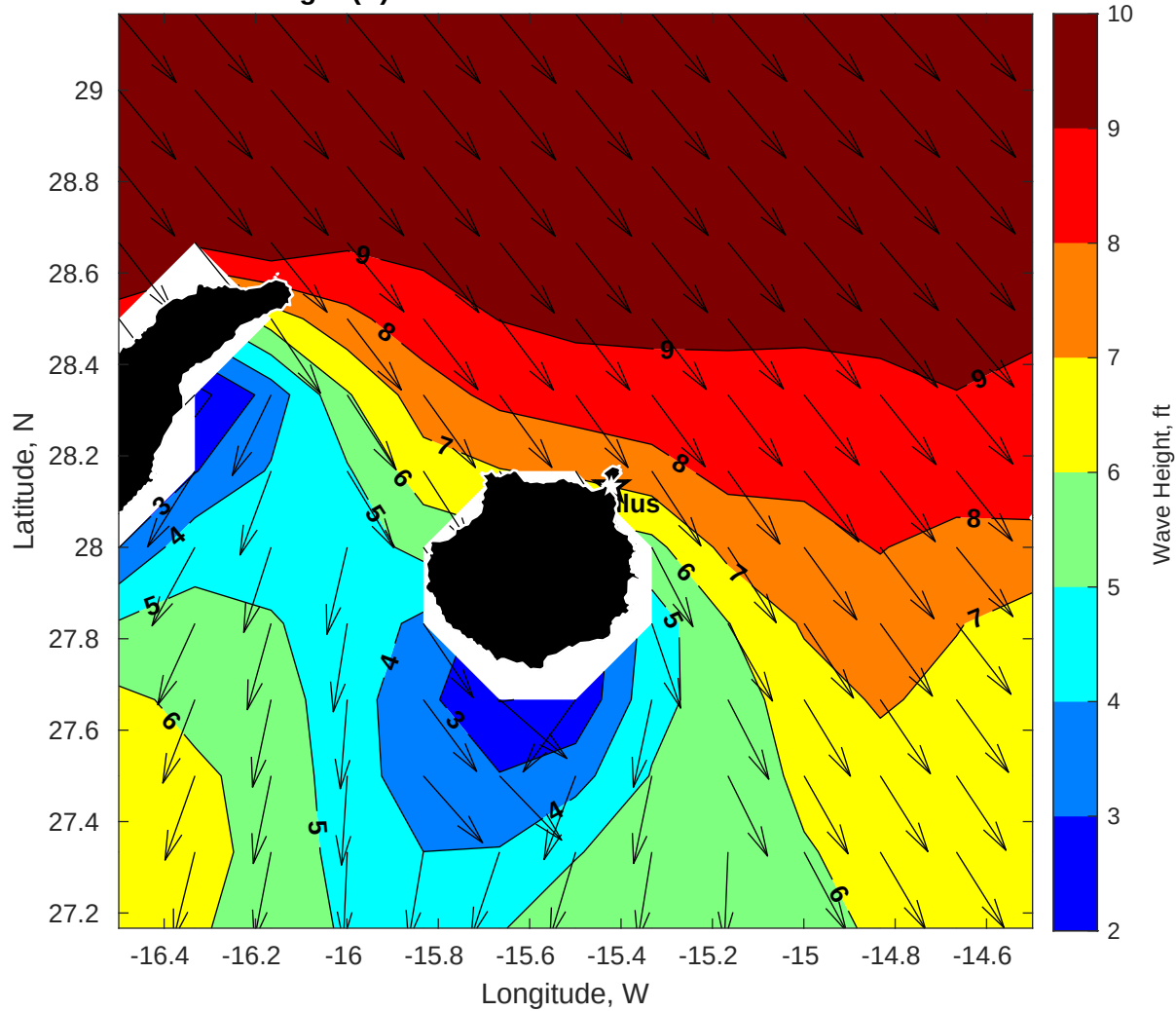
GFS Wave Height (ft) for Nautilus at 14-Jan-2026 09:00:00
