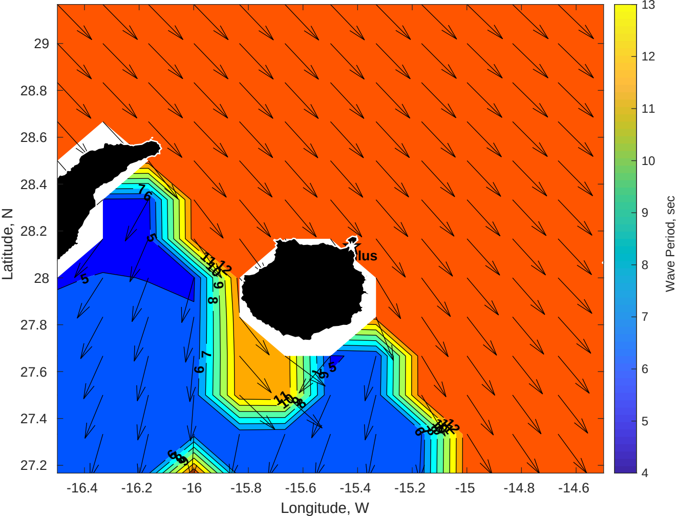
GFS Wave Period (sec) for Nautilus at 14-Jan-2026 09:00:00
