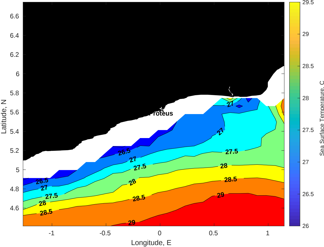
SST for Proteus at 13-Jan-2026 00:00:00
