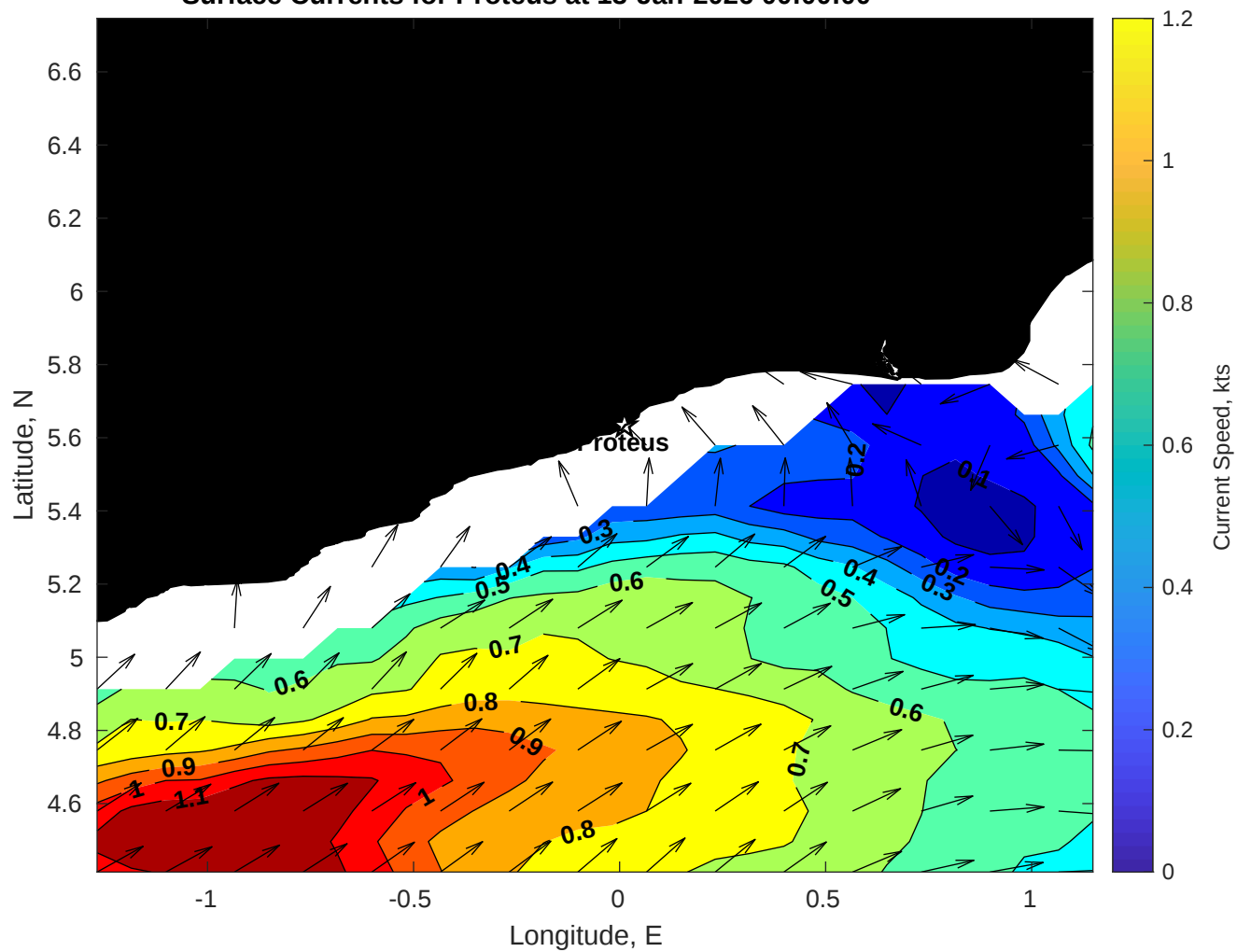
Surface Currents for Proteus at 13-Jan-2026 00:00:00
