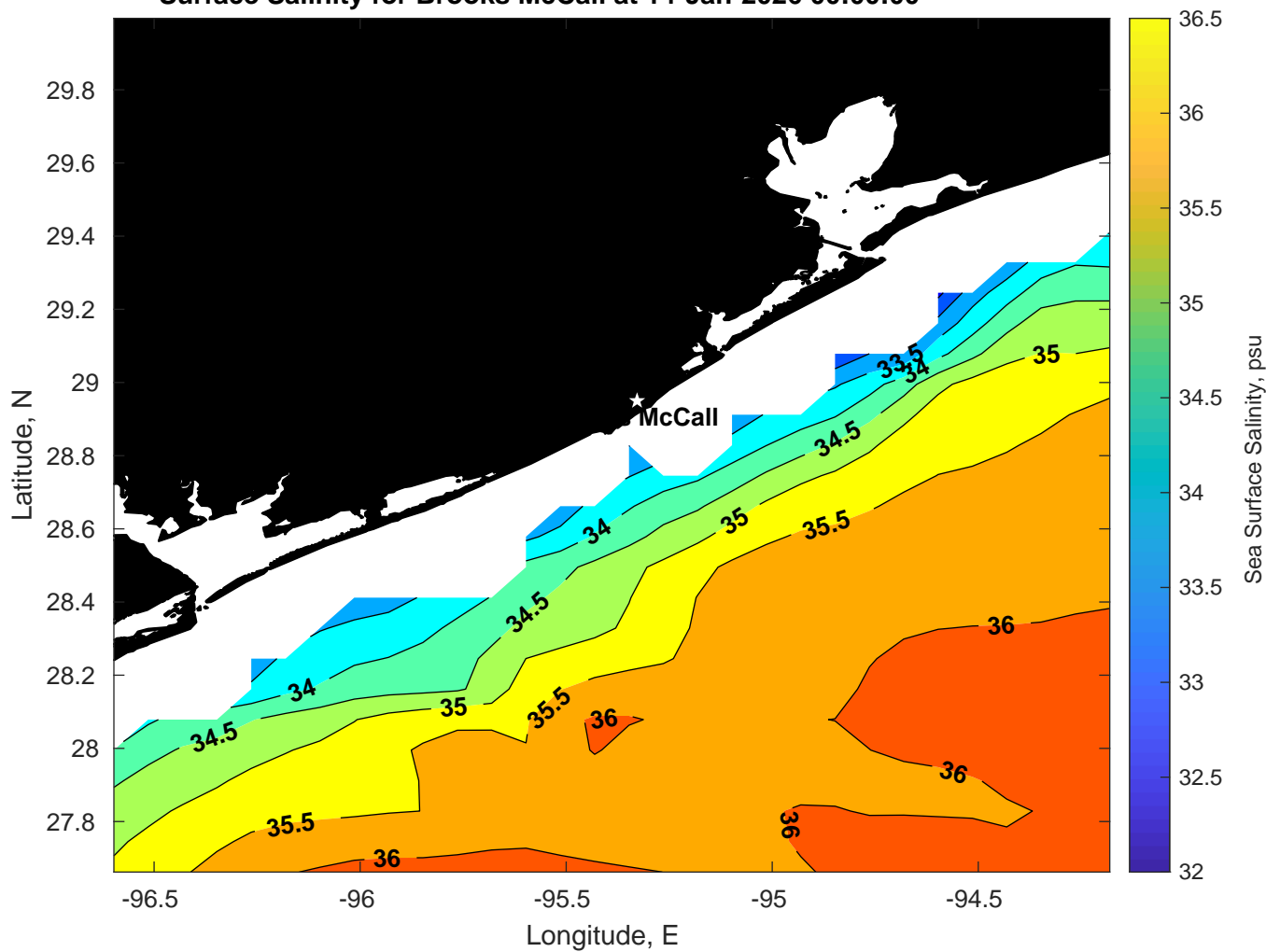
Surface Salinity for Brooks McCall at 14-Jan-2026 00:00:00
