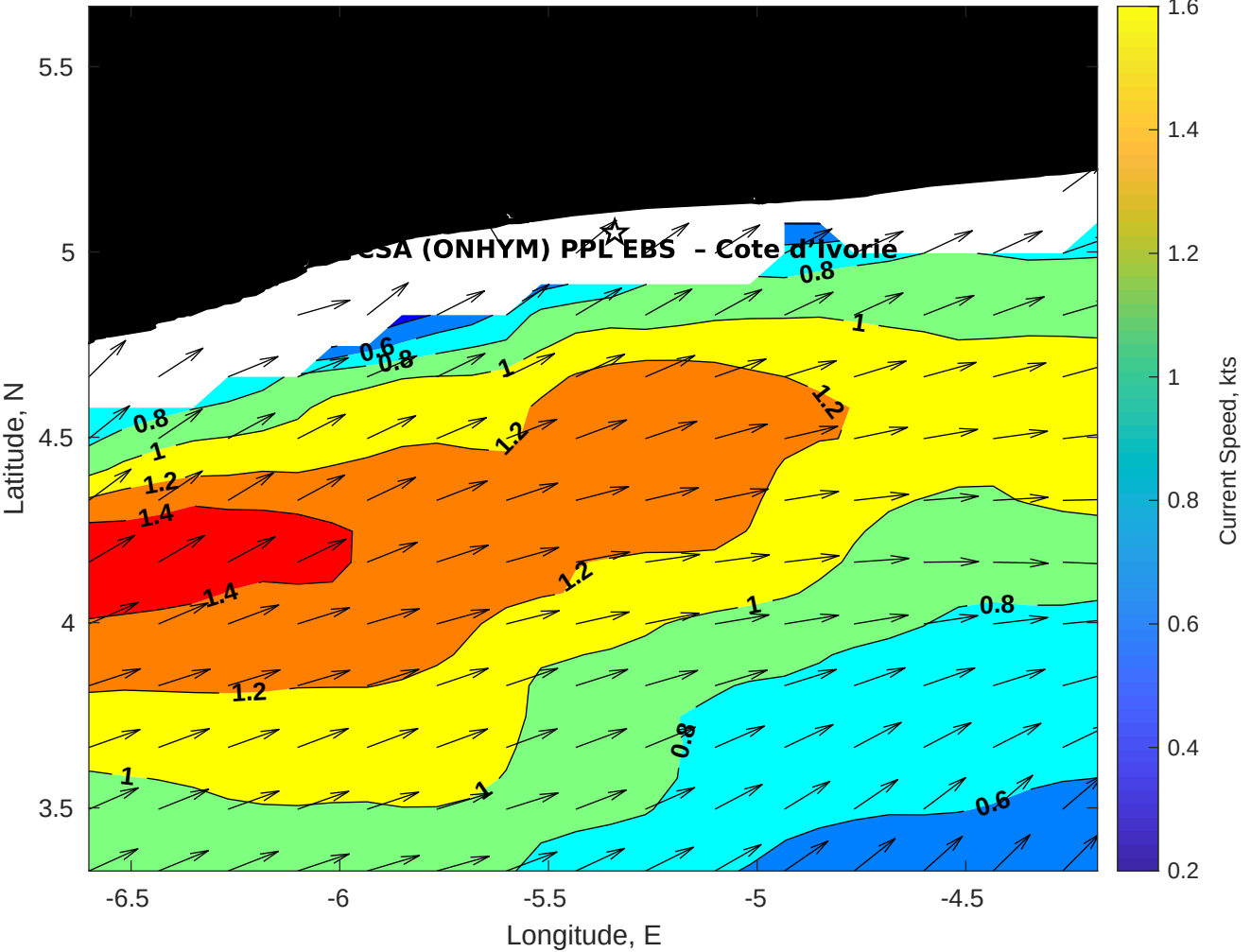
Surface Currents for CSA (ONHYM) PPL EBS - Cote d'Ivoire at 14-Jan-2026 00:00:00
