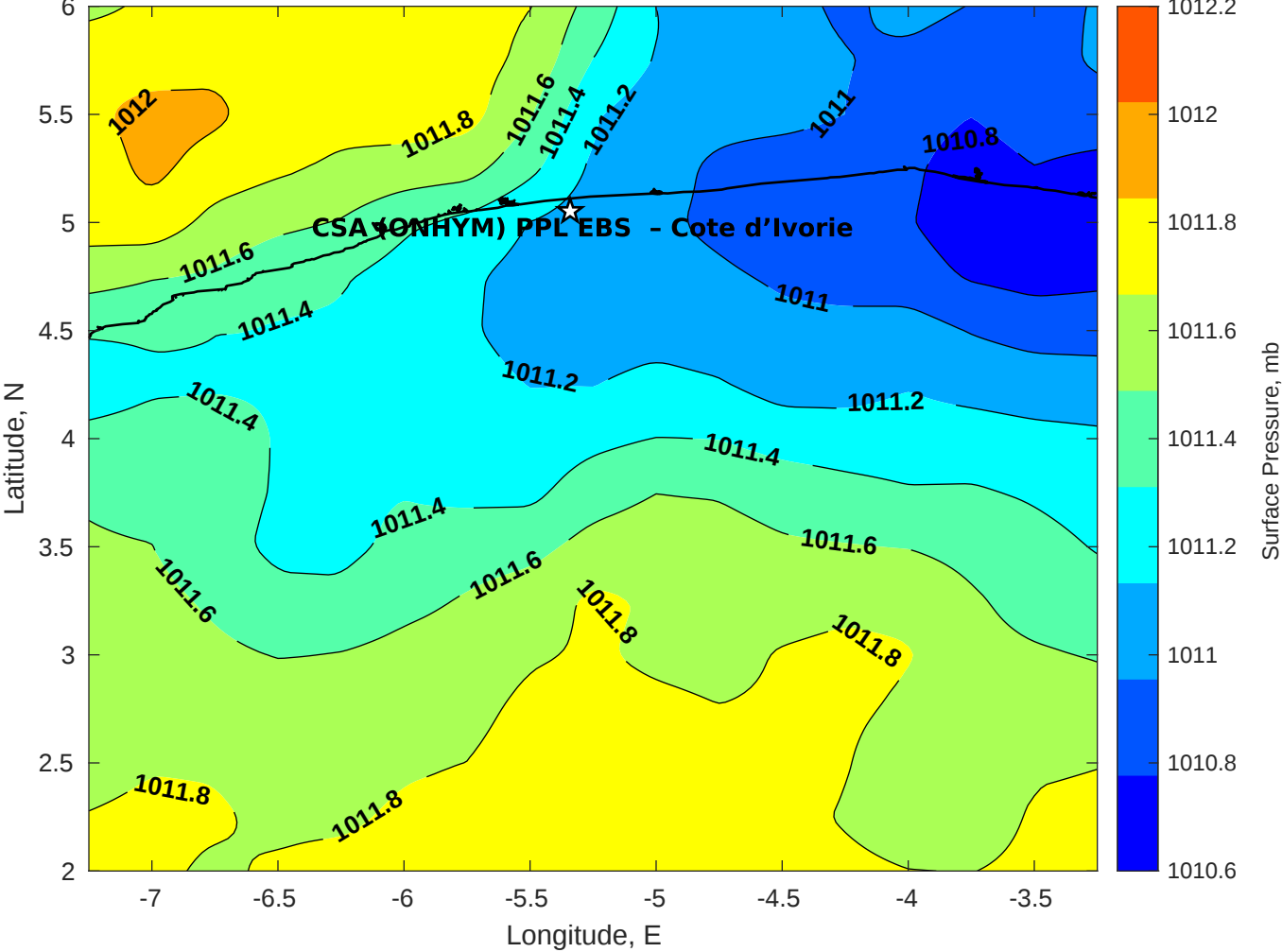
Surface Pressure (mb) for CSA (ONHYM) PPL EBS - Cote d'Ivoire at 15-Jan-2026 00:00:00
