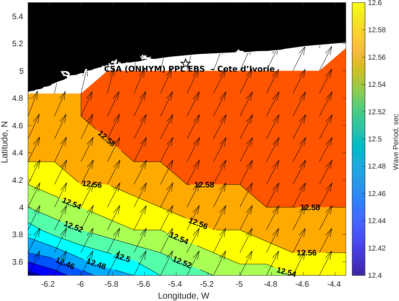
GFS Wave Period (sec) for CSA (ONHYM) PPL EBS - Cote d'Ivoire at 15-Jan-2026 09:00:00
