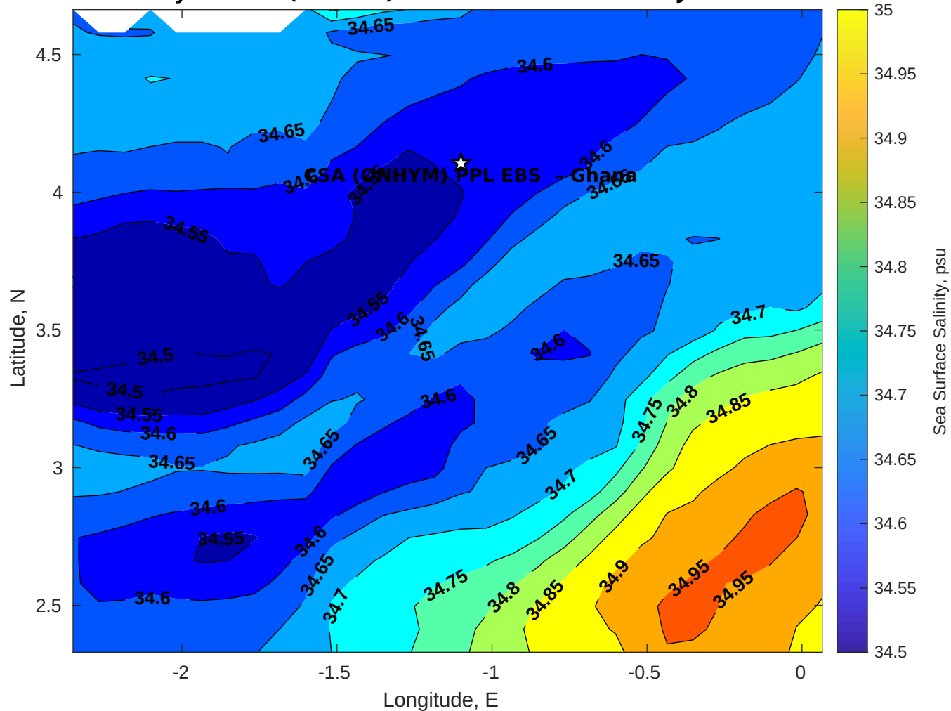
Surface Salinity for CSA (ONHYM) PPL EBS - Ghana at 14-Jan-2026 00:00:00
