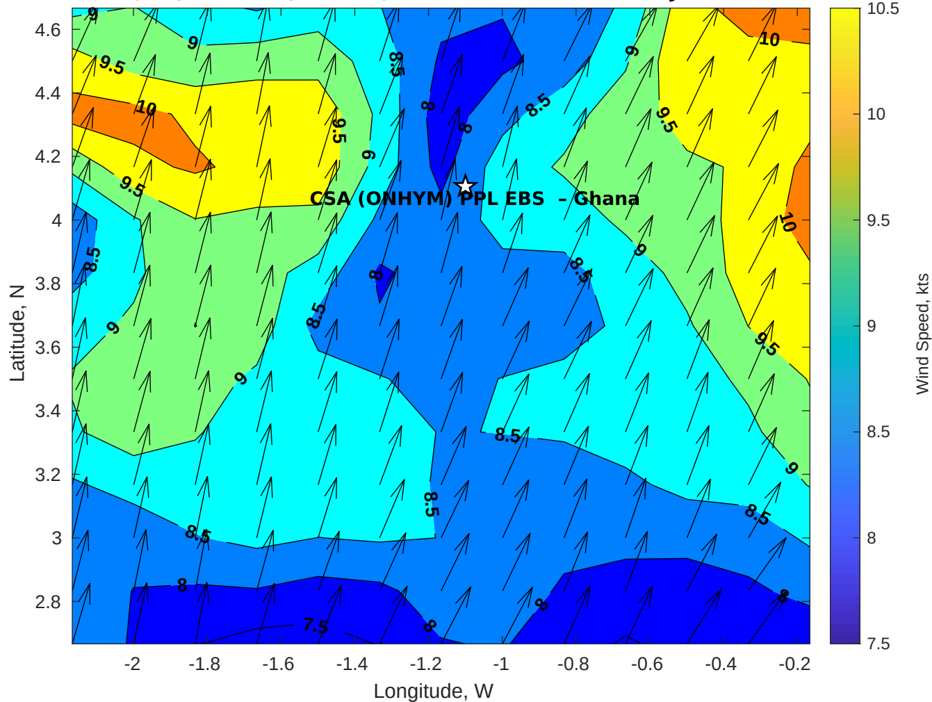
GFS Winds (kts) for CSA (ONHYM) PPL EBS - Ghana at 15-Jan-2026 09:00:00
