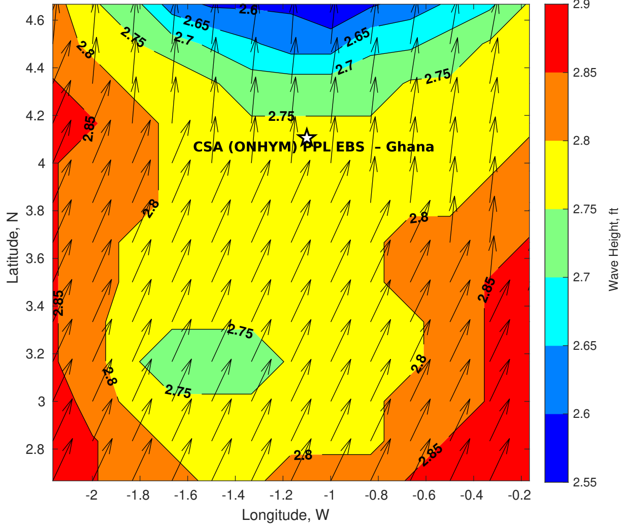
GFS Wave Height (ft) for CSA (ONHYM) PPL EBS - Ghana at 15-Jan-2026 09:00:00
