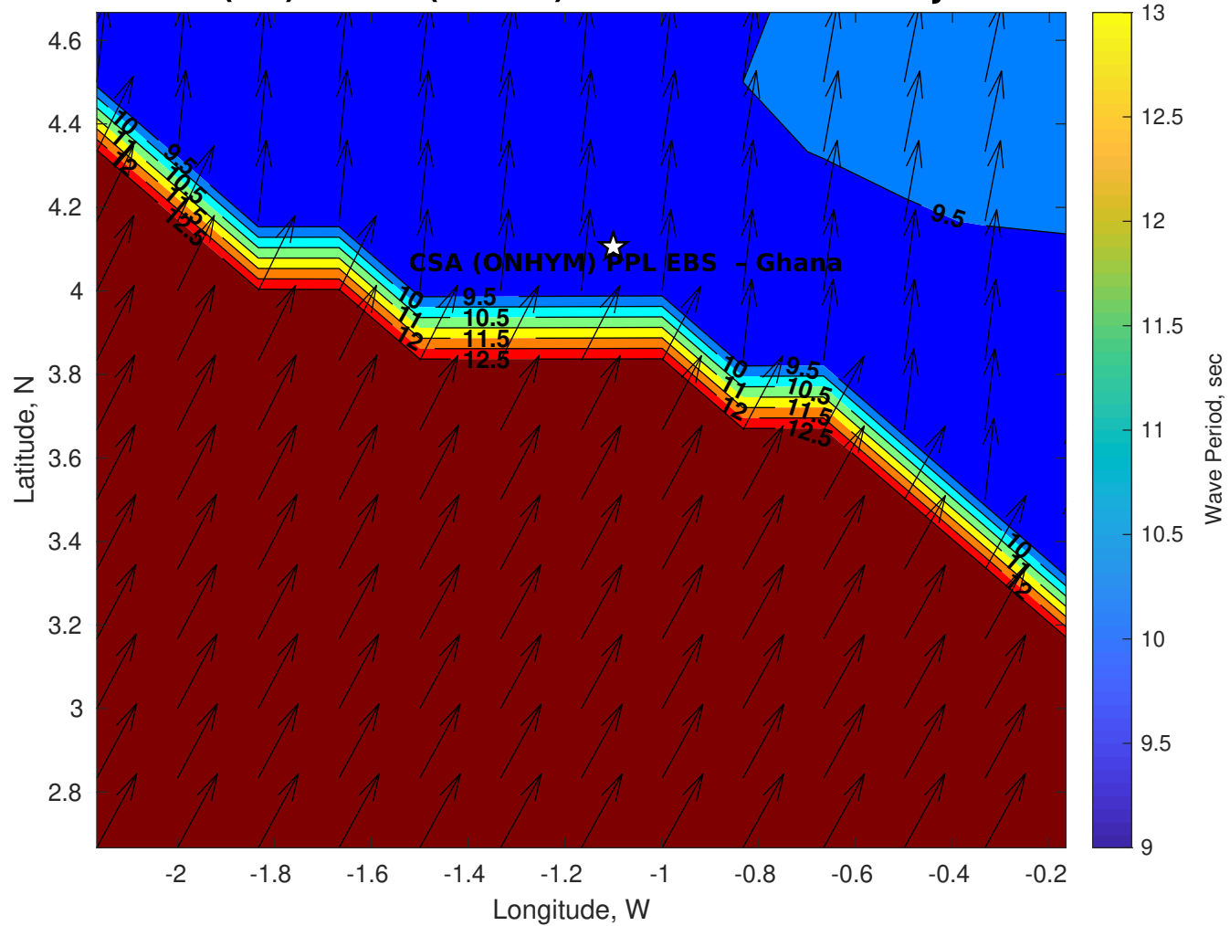
GFS Wave Period (sec) for CSA (ONHYM) PPL EBS - Ghana at 15-Jan-2026 09:00:00
