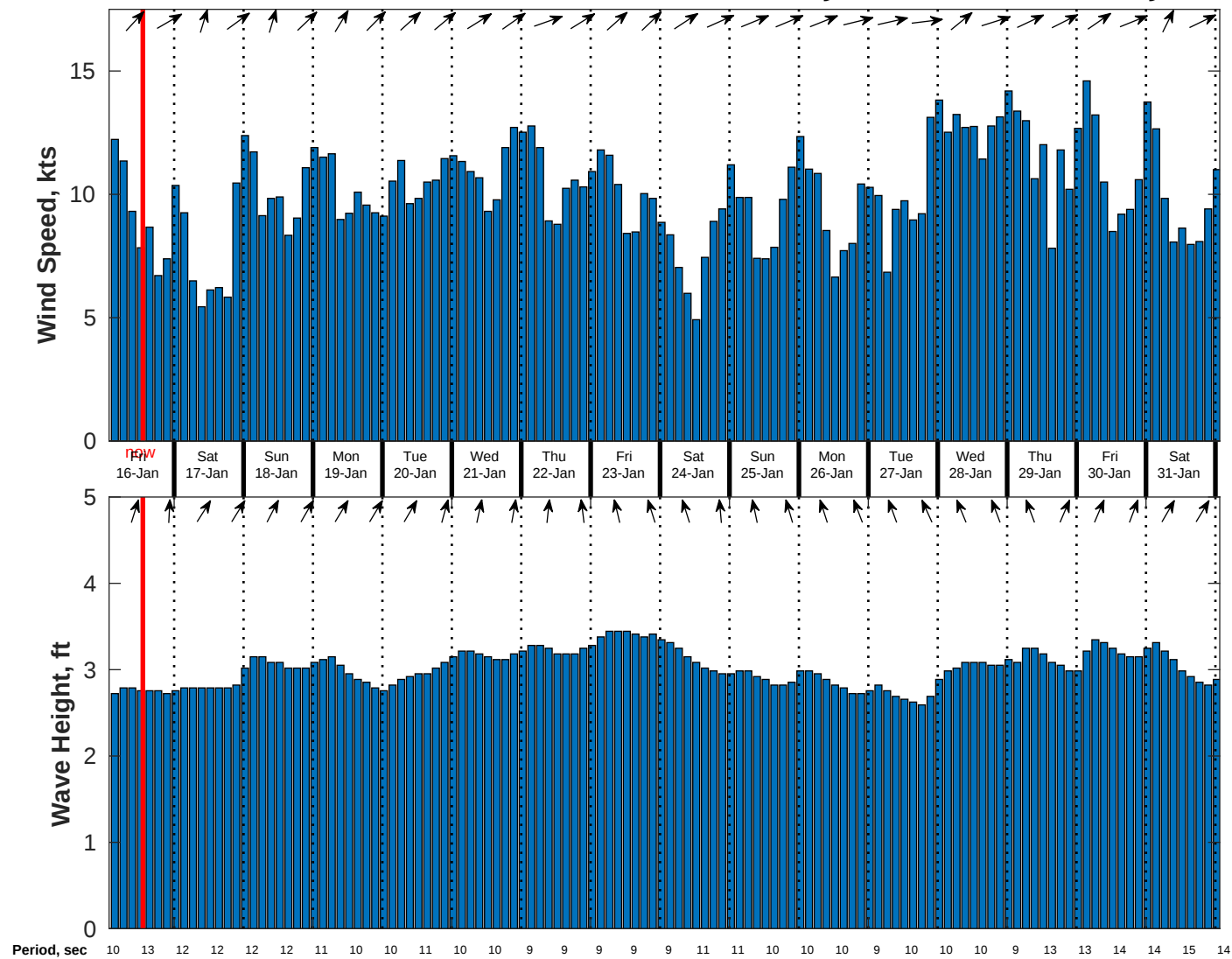
Wind & Wave Forecast for CSA (ONHYM) PPL EBS - Ghana from 15-Jan-2026 02:00:00 to 31-Jan-2026 02:00:00
