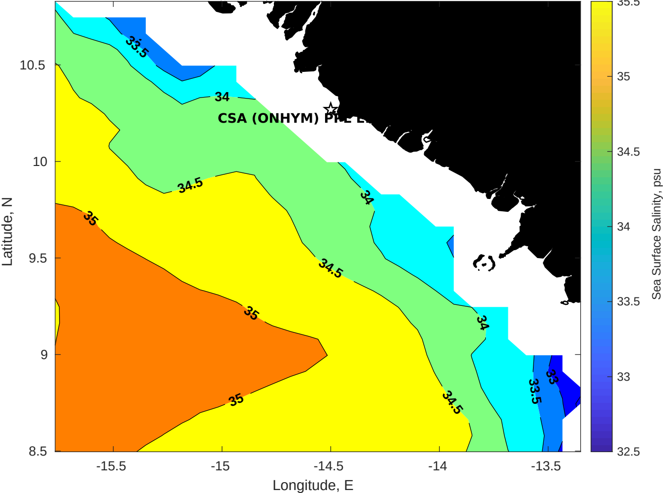
Surface Salinity for CSA (ONHYM) PPL EBS - Guinea at 14-Jan-2026 00:00:00
