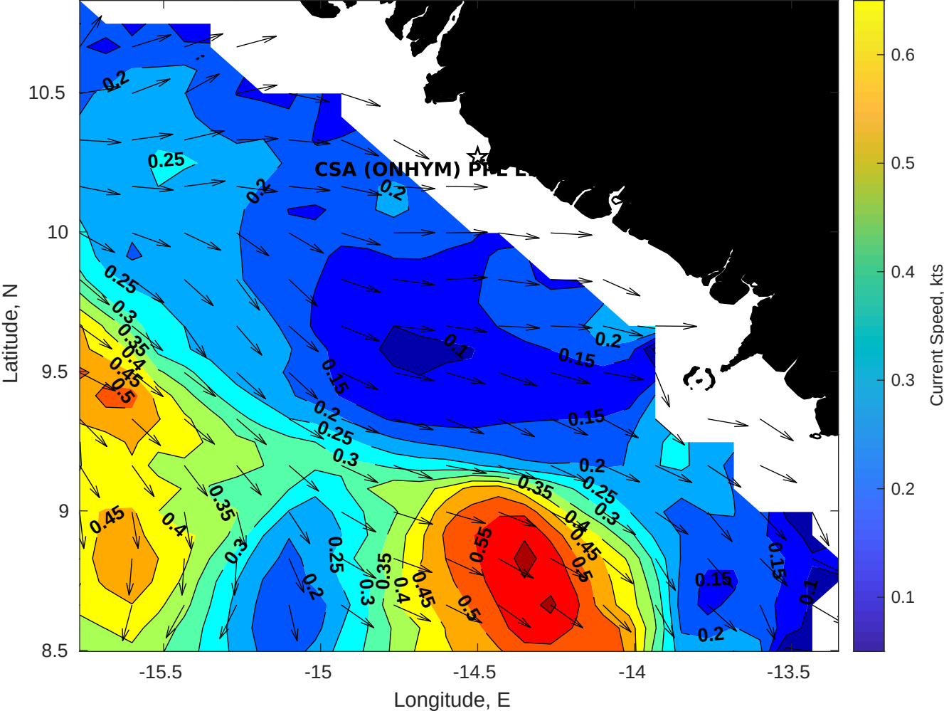
Surface Currents for CSA (ONHYM) PPL EBS - Guinea at 14-Jan-2026 00:00:00
