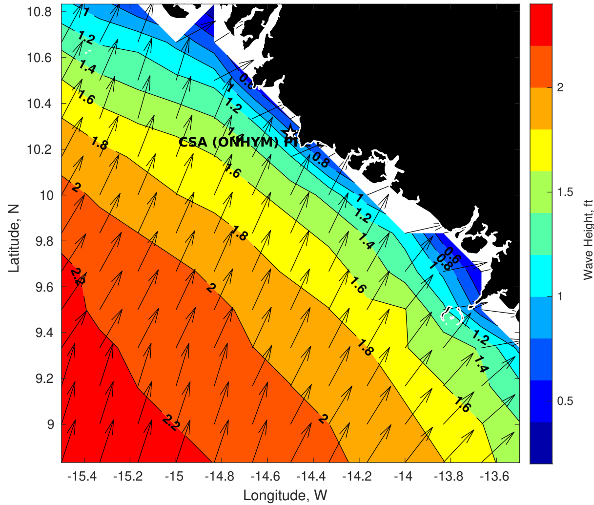
GFS Wave Height (ft) for CSA (ONHYM) PPL EBS - Guinea at 15-Jan-2026 09:00:00
