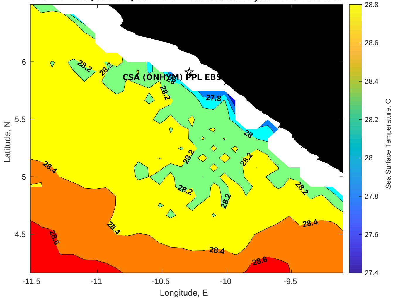
SST for CSA (ONHYM) PPL EBS - Liberia at 14-Jan-2026 00:00:00
