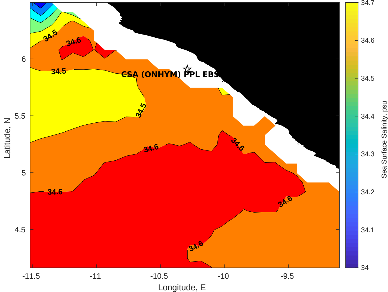
Surface Salinity for CSA (ONHYM) PPL EBS - Liberia at 14-Jan-2026 00:00:00
