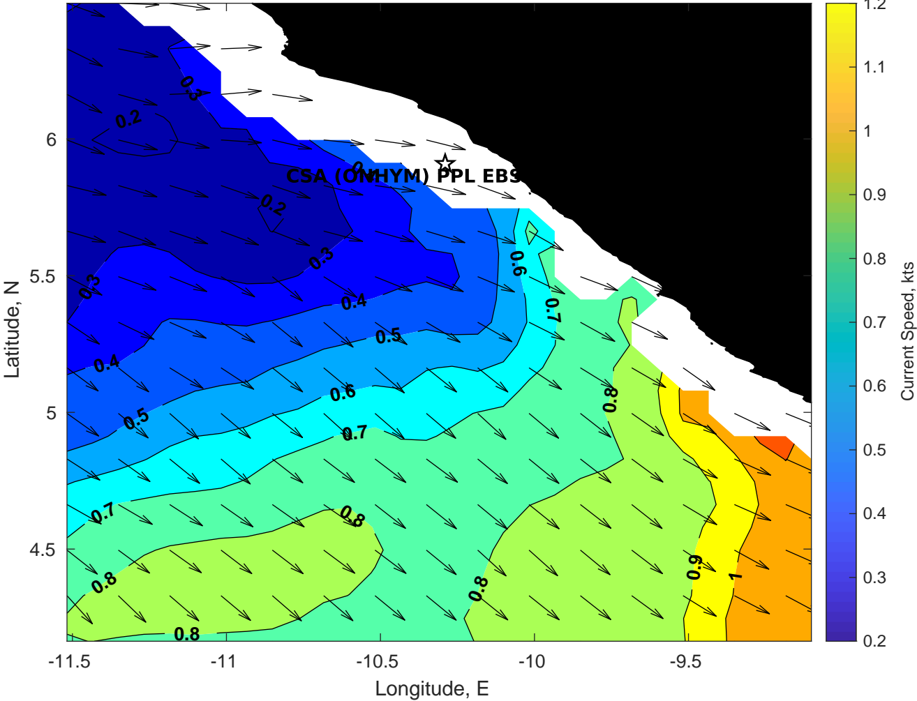
Surface Currents for CSA (ONHYM) PPL EBS - Liberia at 14-Jan-2026 00:00:00
