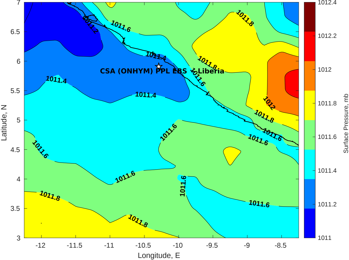
Surface Pressure (mb) for CSA (ONHYM) PPL EBS - Liberia at 17-Jan-2026 00:00:00
