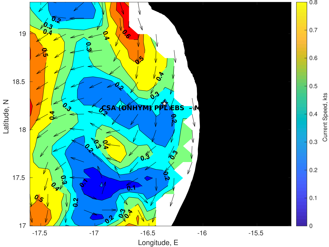
Surface Currents for CSA (ONHYM) PPL EBS - Mauritania at 14-Jan-2026 00:00:00
