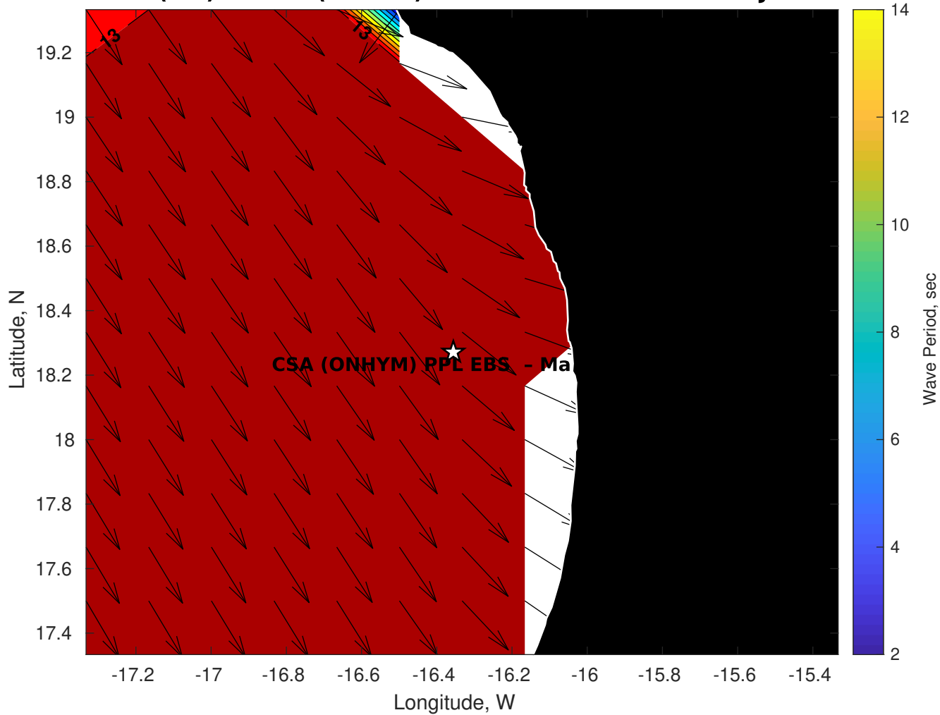
GFS Wave Period (sec) for CSA (ONHYM) PPL EBS - Mauritania at 15-Jan-2026 09:00:00
