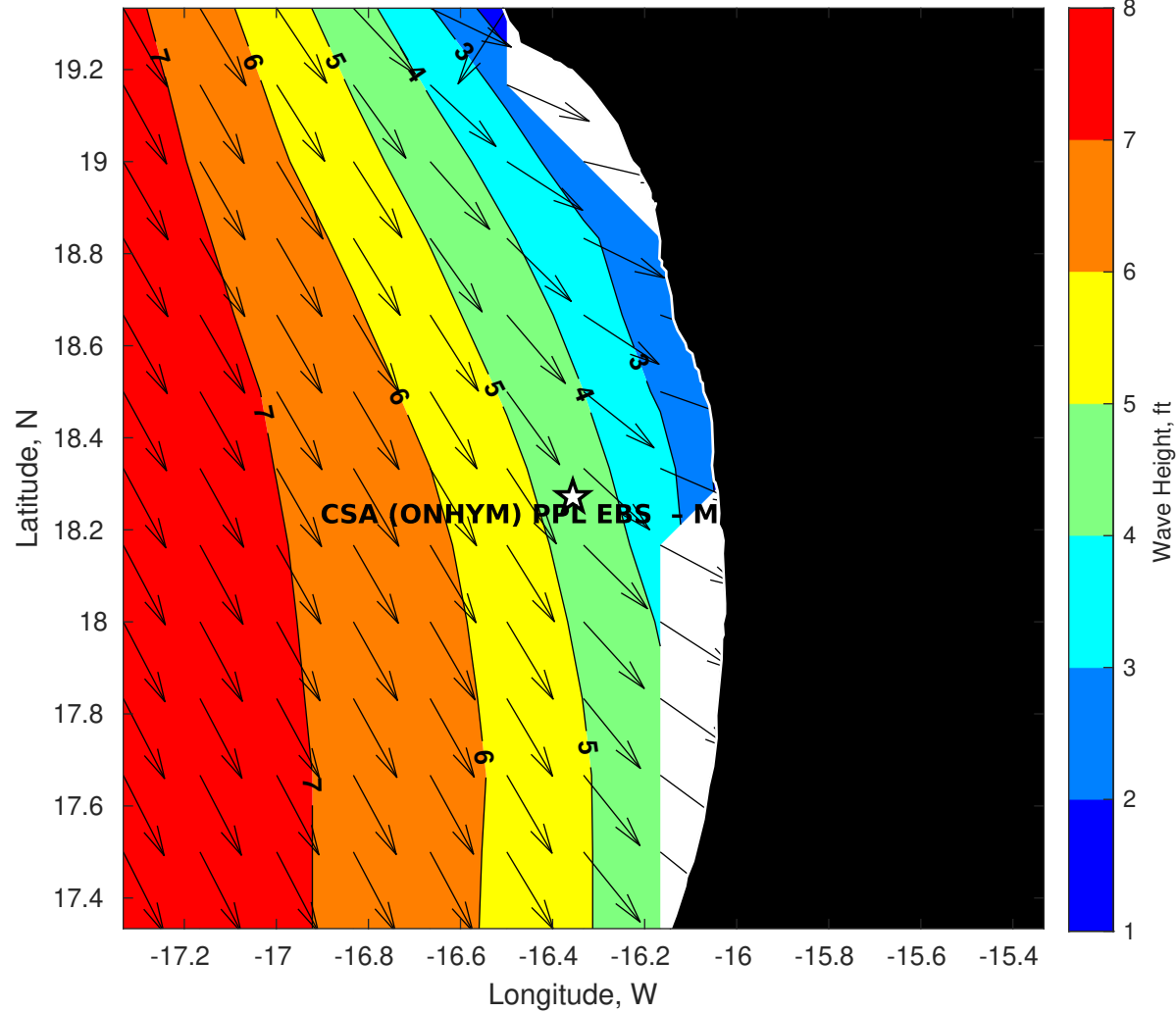
GFS Wave Height (ft) for CSA (ONHYM) PPL EBS - Mauritania at 15-Jan-2026 09:00:00
