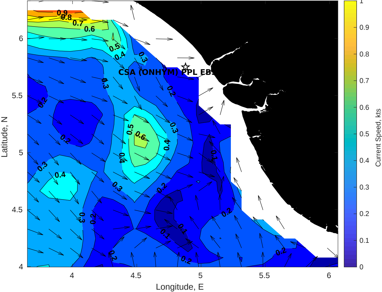
Surface Currents for CSA (ONHYM) PPL EBS - Nigeria at 14-Jan-2026 00:00:00
