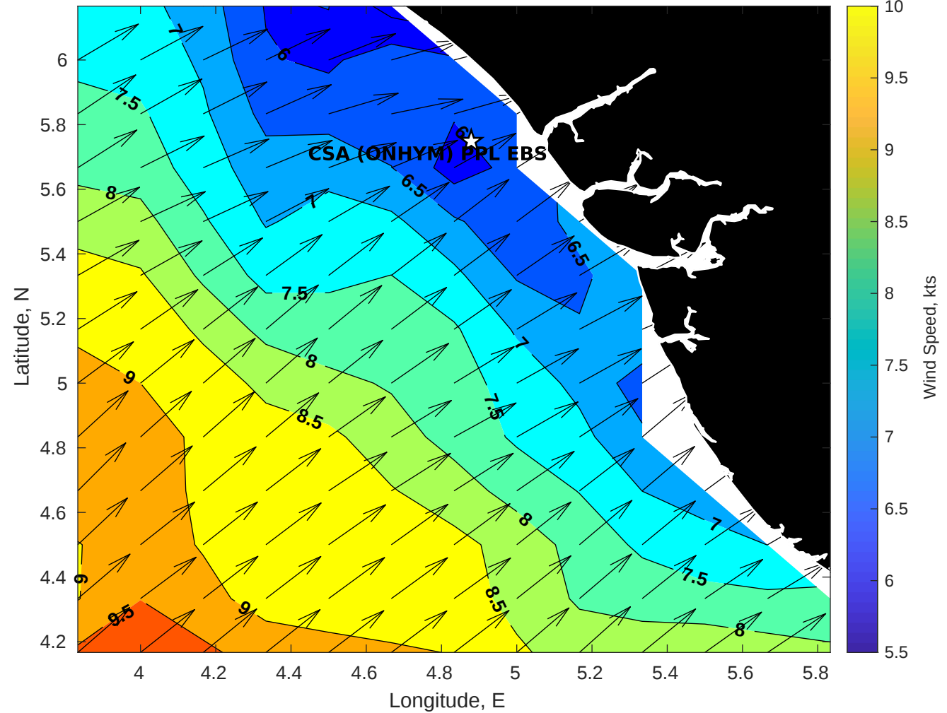
GFS Winds (kts) for CSA (ONHYM) PPL EBS - Nigeria at 15-Jan-2026 09:00:00
