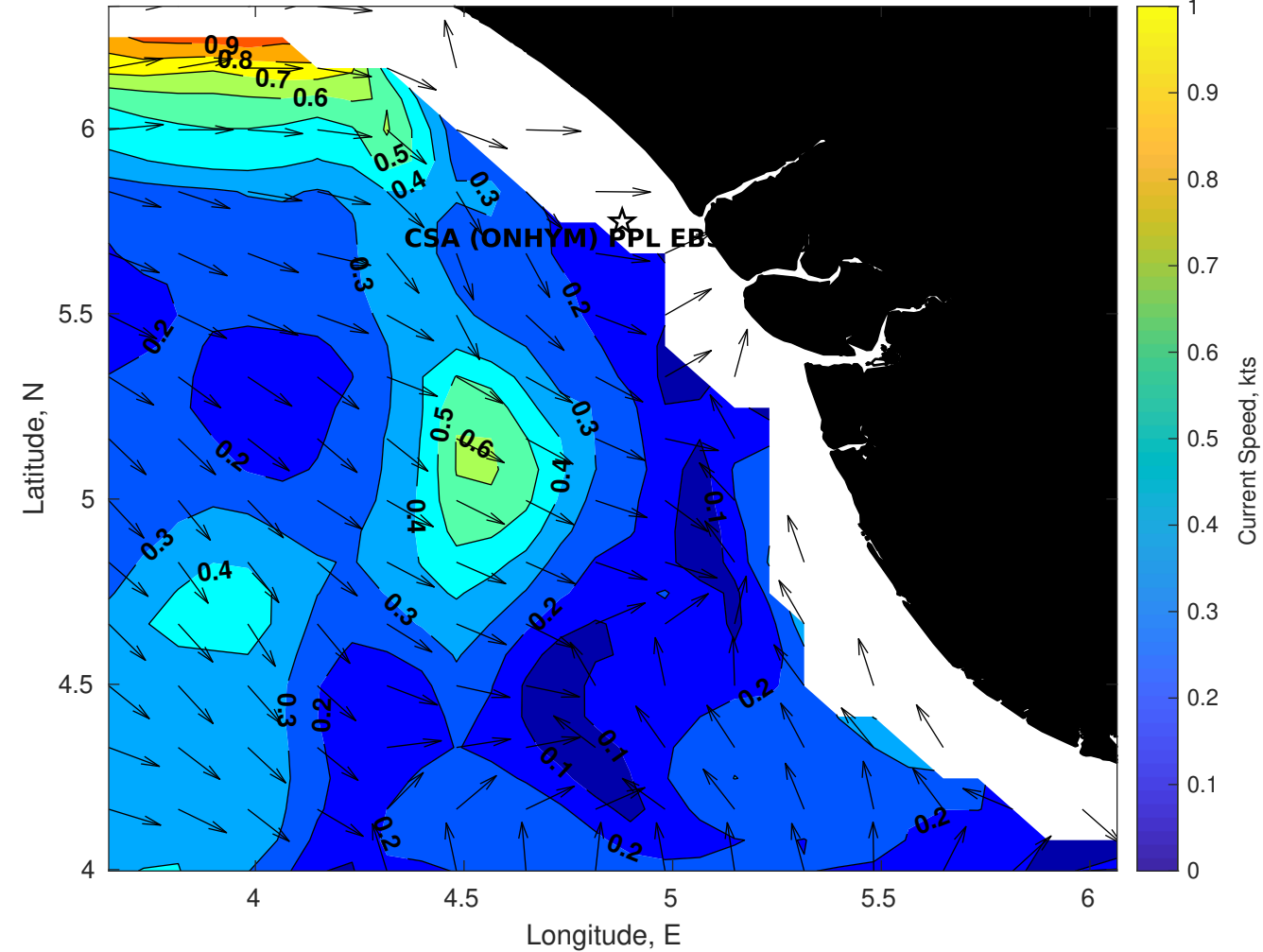
Surface Currents for CSA (ONHYM) PPL EBS - Nigeria at 14-Jan-2026 00:00:00
