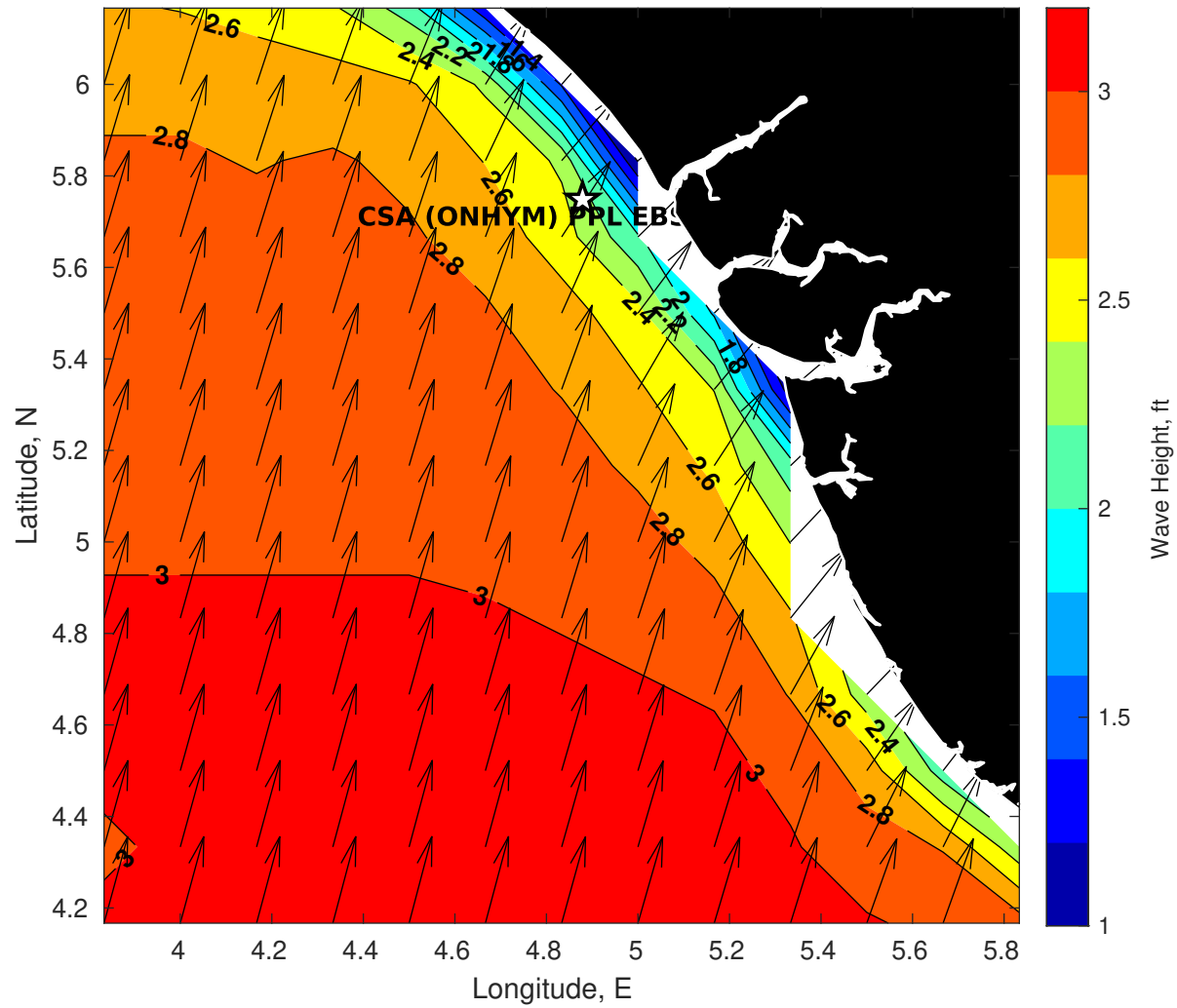
GFS Wave Height (ft) for CSA (ONHYM) PPL EBS - Nigeria at 15-Jan-2026 09:00:00
