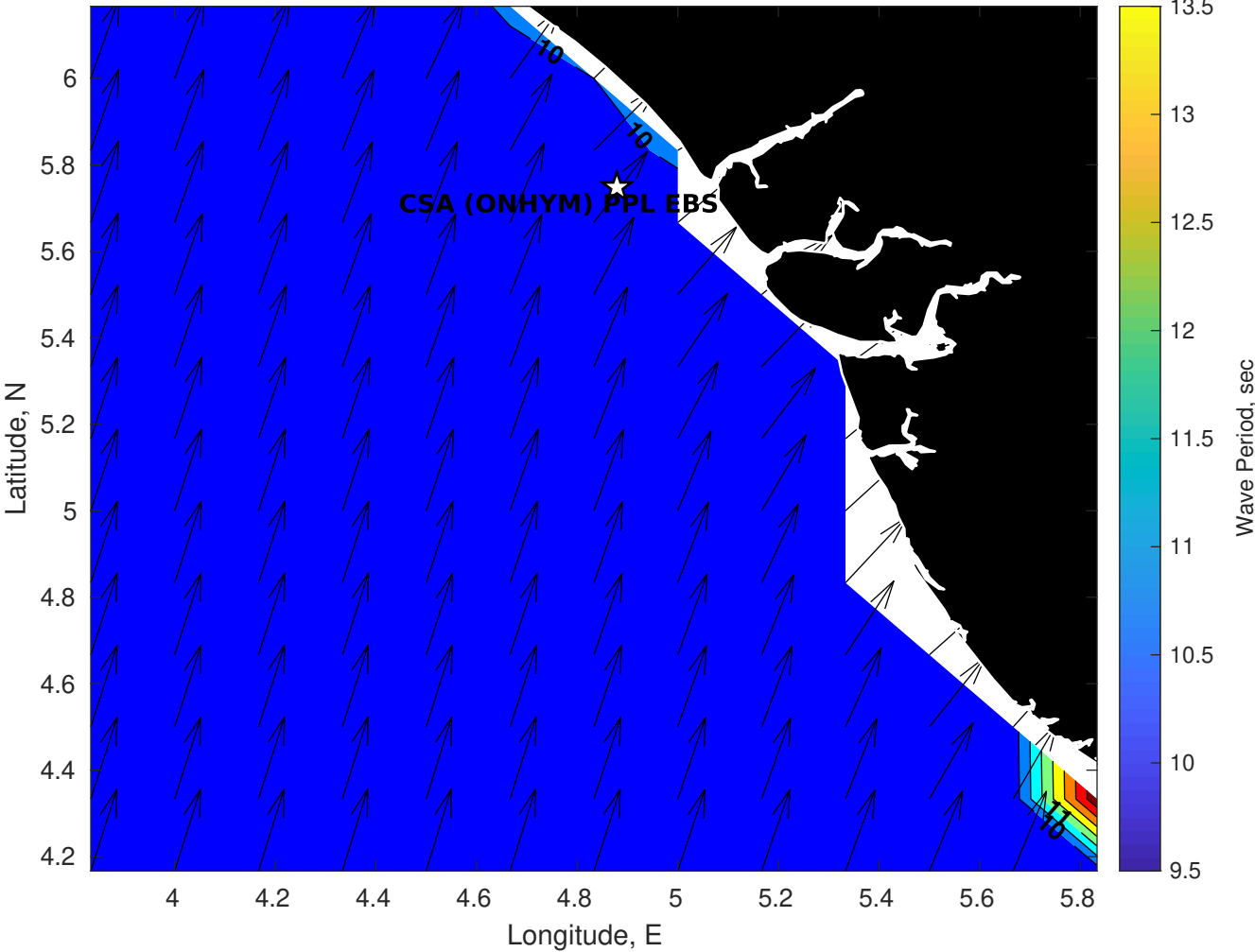
GFS Wave Period (sec) for CSA (ONHYM) PPL EBS - Nigeria at 15-Jan-2026 09:00:00
