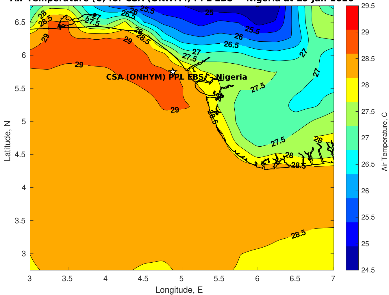
Air Temperature (C) for CSA (ONHYM) PPL EBS - Nigeria at 15-Jan-2026
