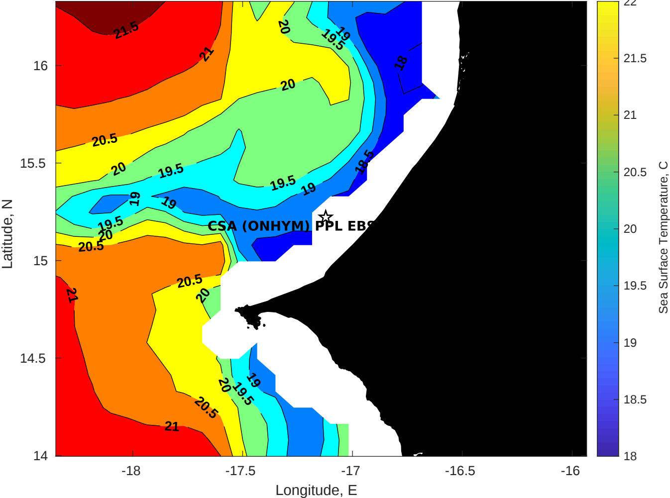
SST for CSA (ONHYM) PPL EBS - Senegal at 14-Jan-2026 00:00:00
