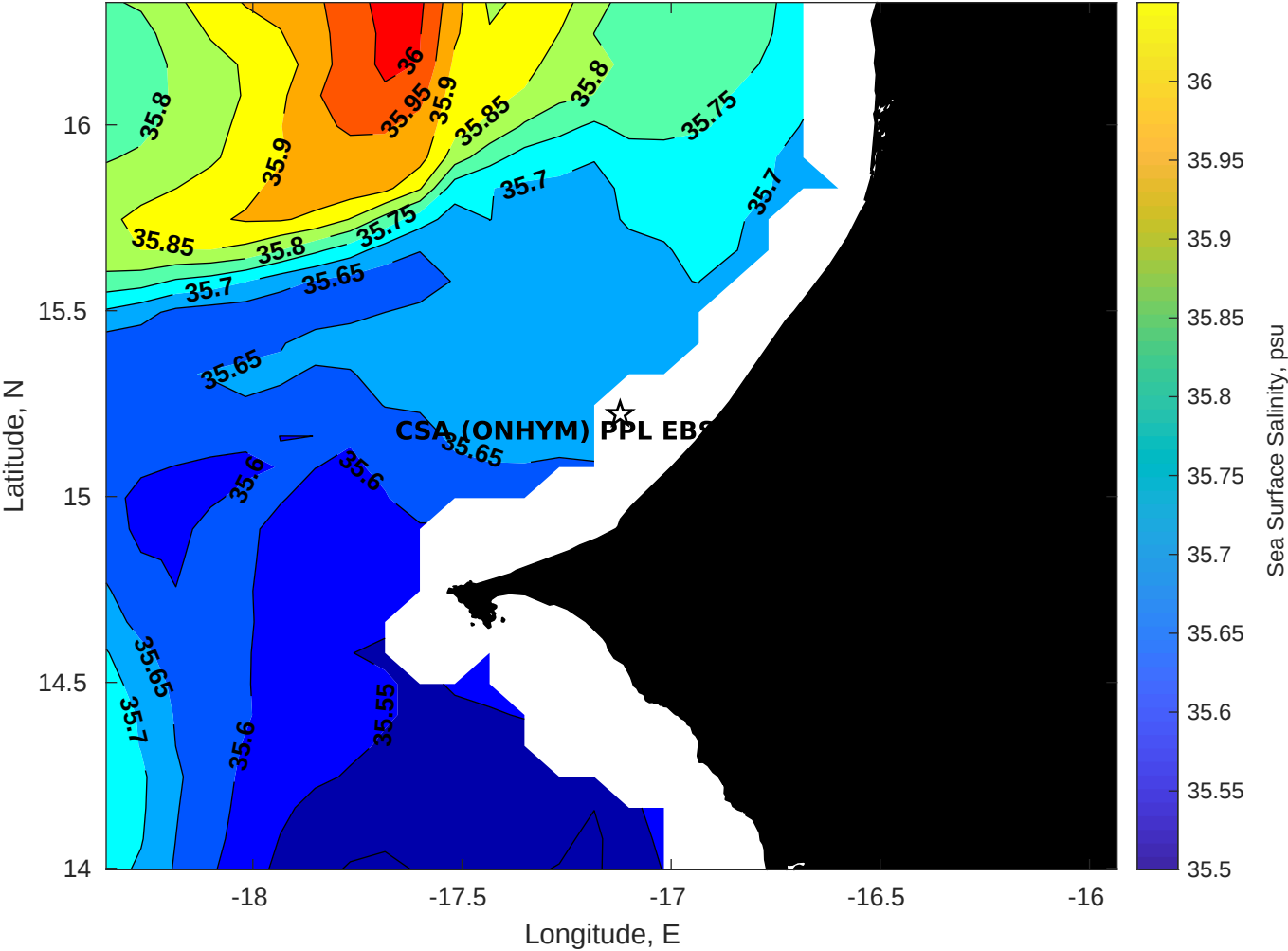
Surface Salinity for CSA (ONHYM) PPL EBS - Senegal at 14-Jan-2026 00:00:00
